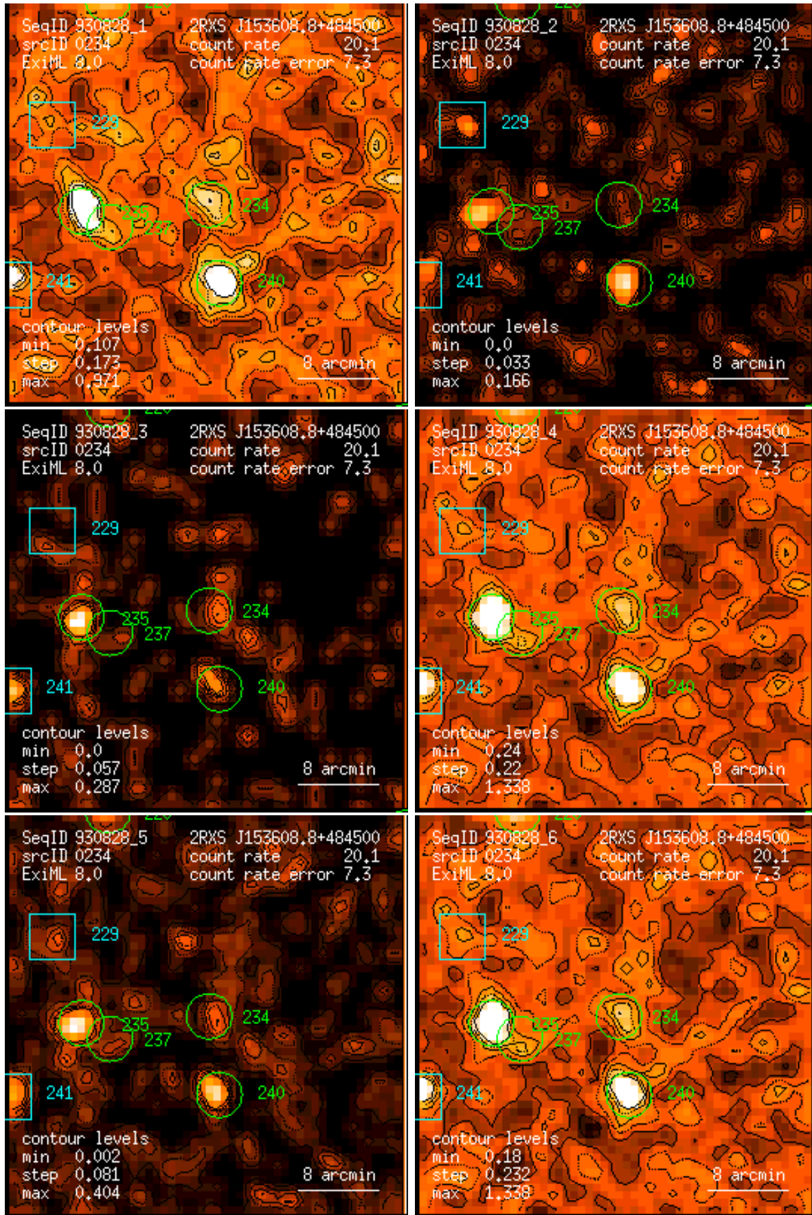
Figure 234: RASS 930828: detection 0234: band rate images, Gaussian filter: (1) PSPC channels 11 – 41, (2) 52 – 90, (3) 91 – 201, (4) 11 – 235, (5) 52 – 201, (6) 11 – 201. Broad band rates in counts/ks. Band rate contour levels in counts/ks/arcmin 2 .
