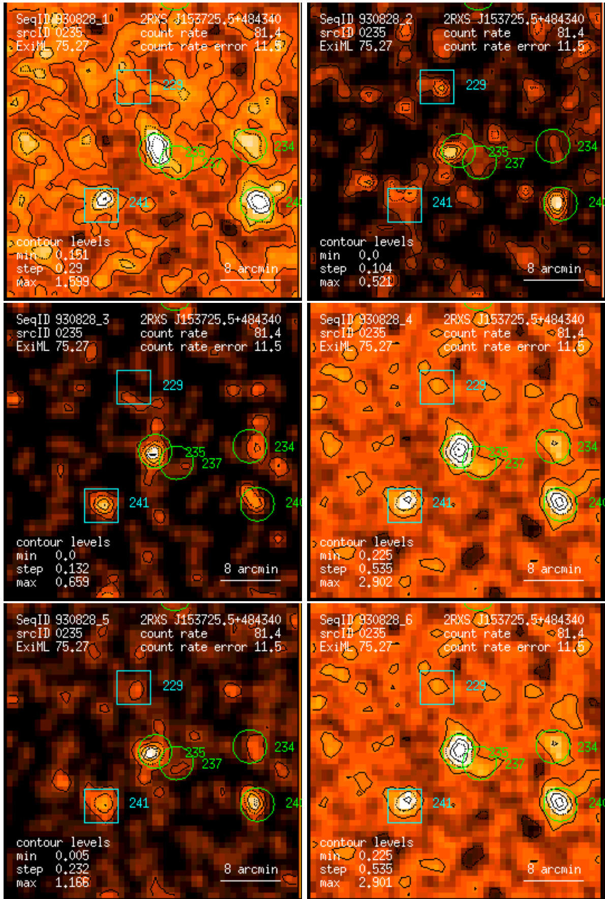
Figure 235: RASS 930828: detection 0235: band rate images, Gaussian filter: (1) PSPC channels 11 – 41, (2) 52 – 90, (3) 91 – 201, (4) 11 – 235, (5) 52 – 201, (6) 11 – 201. Broad band rates in counts/ks. Band rate contour levels in counts/ks/arcmin 2 .
