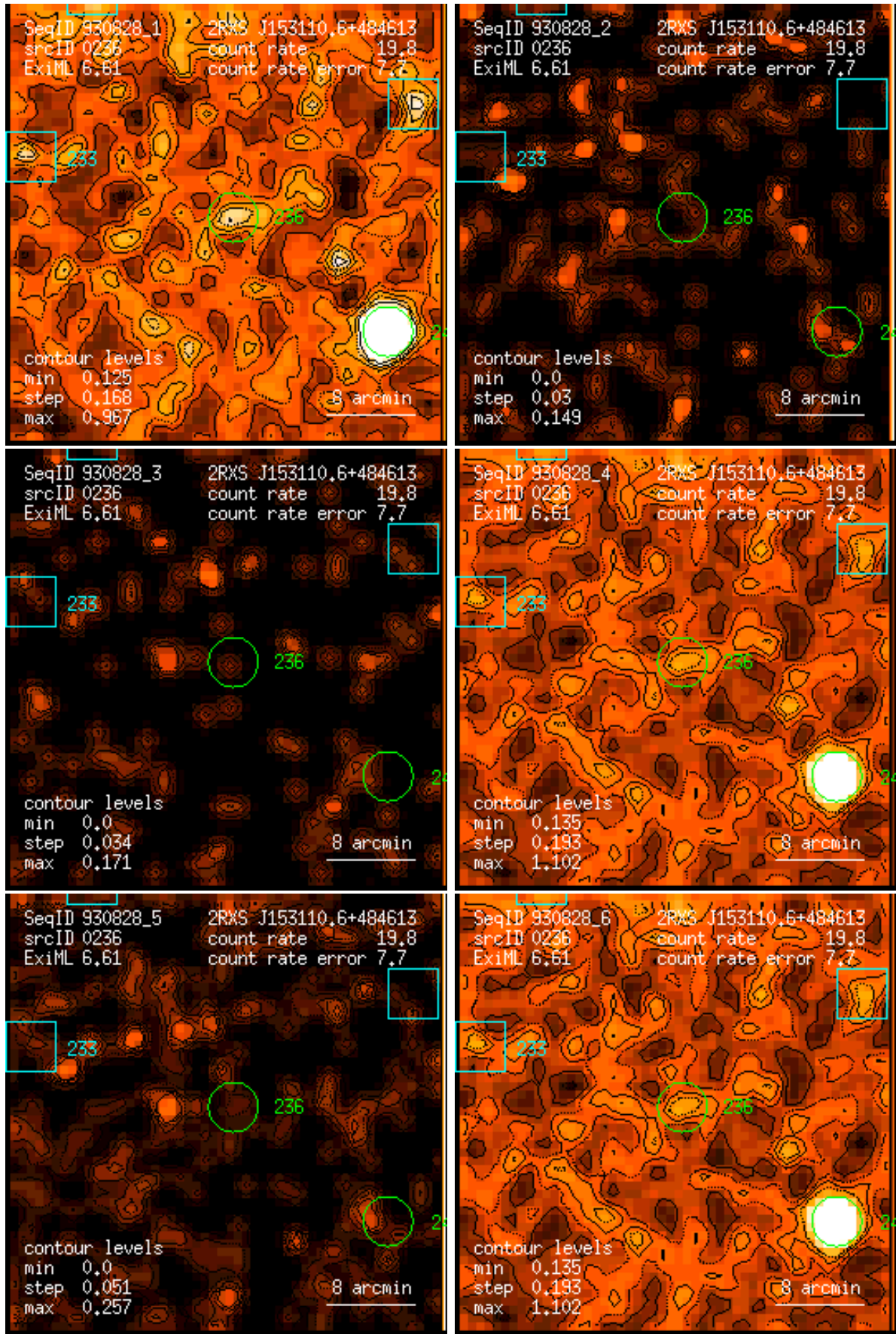
Figure 236: RASS 930828: detection 0236: band rate images, Gaussian filter: (1) PSPC channels 11 – 41, (2) 52 – 90, (3) 91 – 201, (4) 11 – 235, (5) 52 – 201, (6) 11 – 201. Broad band rates in counts/ks. Band rate contour levels in counts/ks/arcmin 2 .
