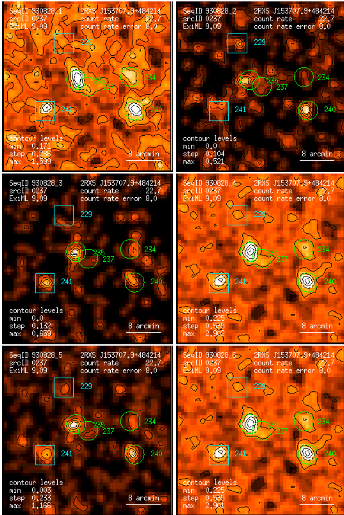
Figure 237: RASS 930828: detection 0237: band rate images, Gaussian filter: (1) PSPC channels 11 – 41, (2) 52 – 90, (3) 91 – 201, (4) 11 – 235, (5) 52 – 201, (6) 11 – 201. Broad band rates in counts/ks. Band rate contour levels in counts/ks/arcmin 2 .
