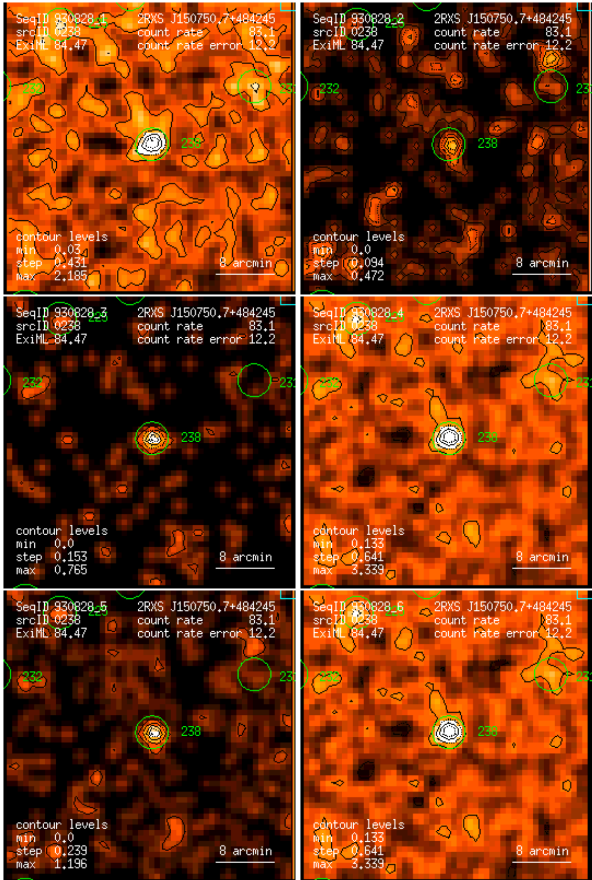
Figure 238: RASS 930828: detection 0238: band rate images, Gaussian filter: (1) PSPC channels 11 – 41, (2) 52 – 90, (3) 91 – 201, (4) 11 – 235, (5) 52 – 201, (6) 11 – 201. Broad band rates in counts/ks. Band rate contour levels in counts/ks/arcmin 2 .
