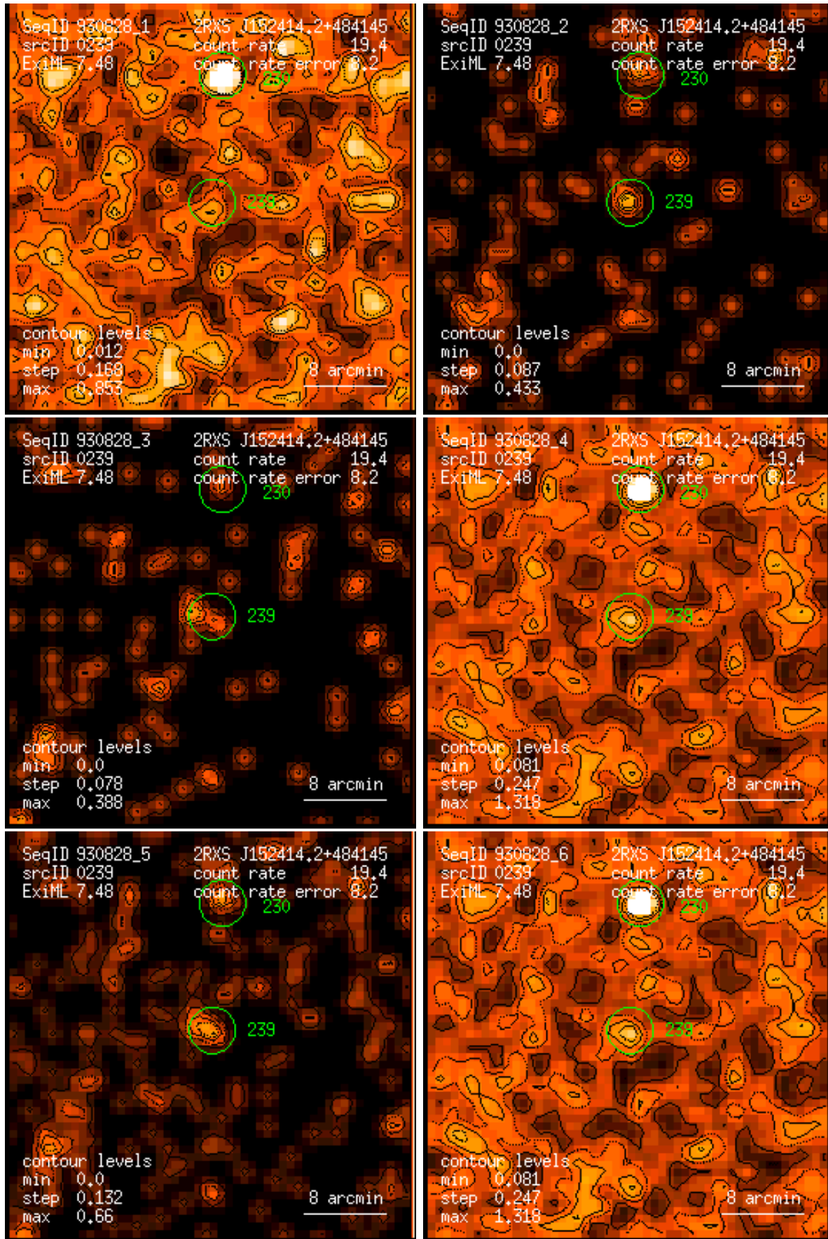
Figure 239: RASS 930828: detection 0239: band rate images, Gaussian filter: (1) PSPC channels 11 – 41, (2) 52 – 90, (3) 91 – 201, (4) 11 – 235, (5) 52 – 201, (6) 11 – 201. Broad band rates in counts/ks. Band rate contour levels in counts/ks/arcmin 2 .
