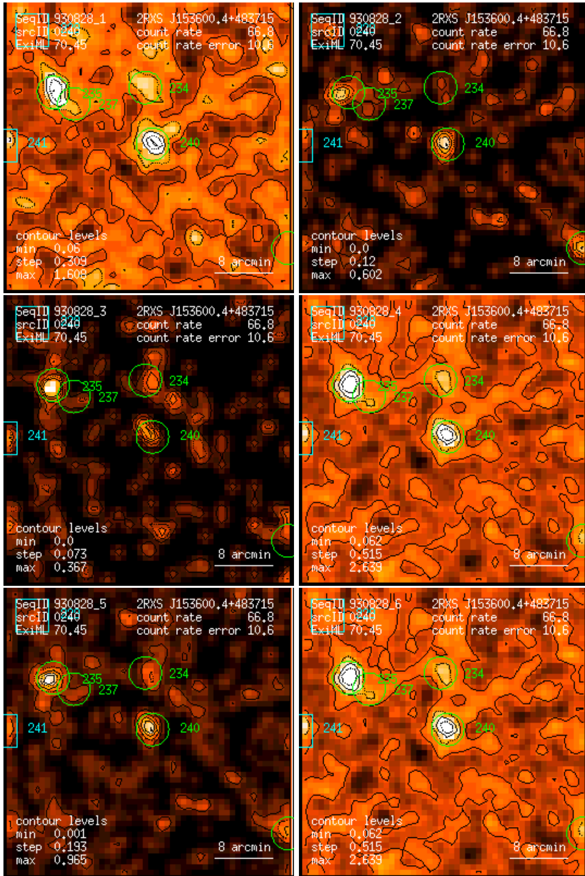
Figure 240: RASS 930828: detection 0240: band rate images, Gaussian filter: (1) PSPC channels 11 – 41, (2) 52 – 90, (3) 91 – 201, (4) 11 – 235, (5) 52 – 201, (6) 11 – 201. Broad band rates in counts/ks. Band rate contour levels in counts/ks/arcmin 2 .
