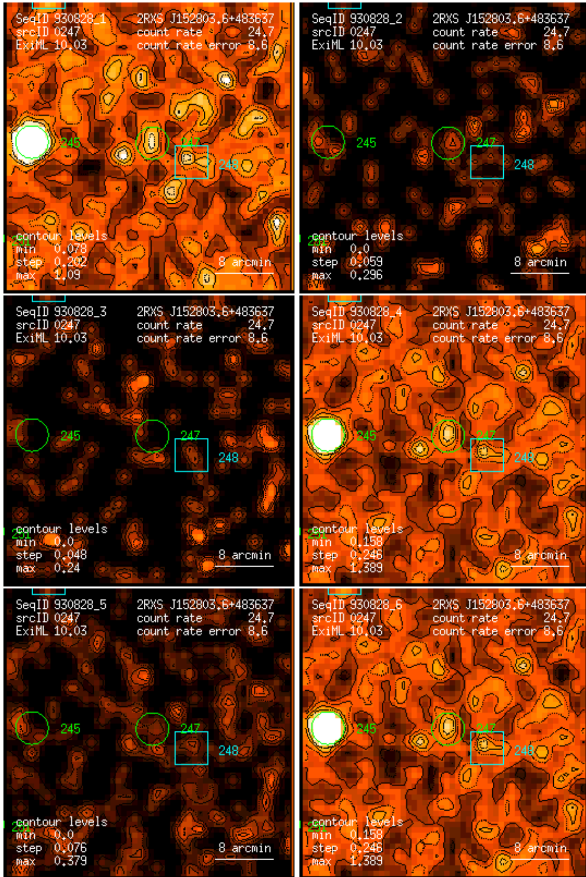
Figure 247: RASS 930828: detection 0247: band rate images, Gaussian filter: (1) PSPC channels 11 – 41, (2) 52 – 90, (3) 91 – 201, (4) 11 – 235, (5) 52 – 201, (6) 11 – 201. Broad band rates in counts/ks. Band rate contour levels in counts/ks/arcmin 2 .
