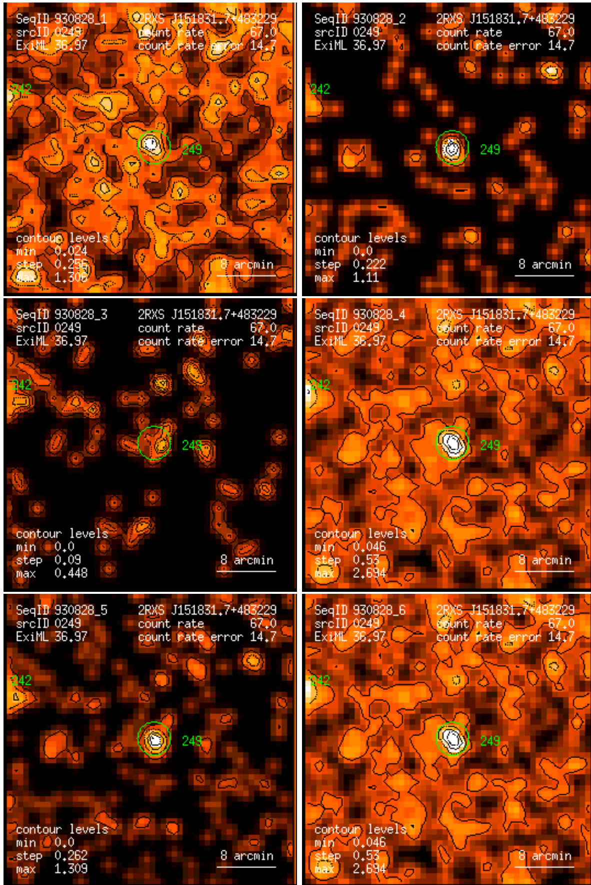
Figure 249: RASS 930828: detection 0249: band rate images, Gaussian filter: (1) PSPC channels 11 – 41, (2) 52 – 90, (3) 91 – 201, (4) 11 – 235, (5) 52 – 201, (6) 11 – 201. Broad band rates in counts/ks. Band rate contour levels in counts/ks/arcmin 2 .
