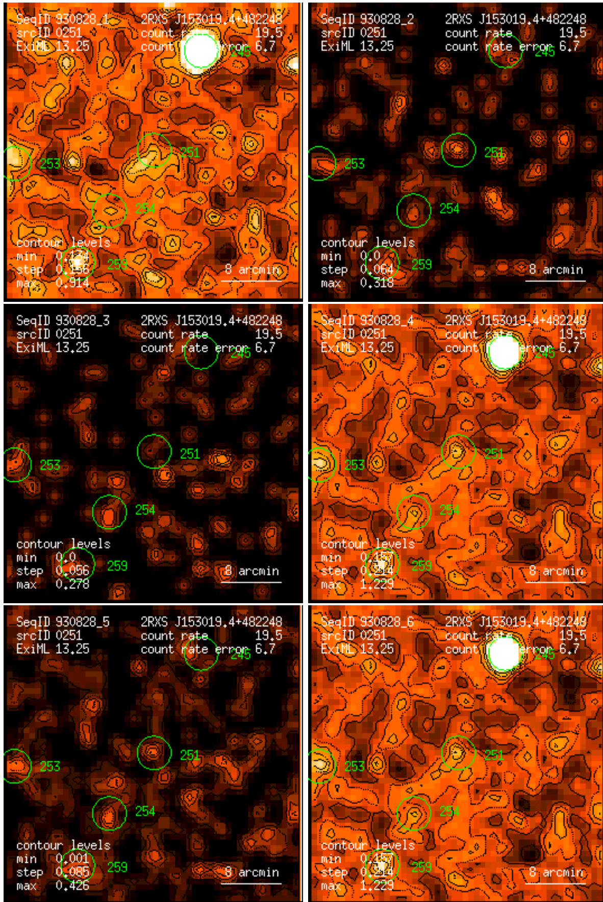
Figure 251: RASS 930828: detection 0251: band rate images, Gaussian filter: (1) PSPC channels 11 – 41, (2) 52 – 90, (3) 91 – 201, (4) 11 – 235, (5) 52 – 201, (6) 11 – 201. Broad band rates in counts/ks. Band rate contour levels in counts/ks/arcmin 2 .
