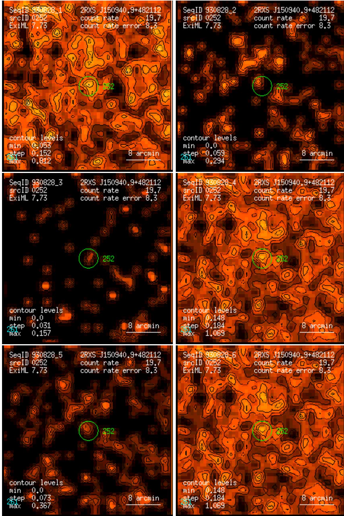
Figure 252: RASS 930828: detection 0252: band rate images, Gaussian filter: (1) PSPC channels 11 – 41, (2) 52 – 90, (3) 91 – 201, (4) 11 – 235, (5) 52 – 201, (6) 11 – 201. Broad band rates in counts/ks. Band rate contour levels in counts/ks/arcmin 2 .
