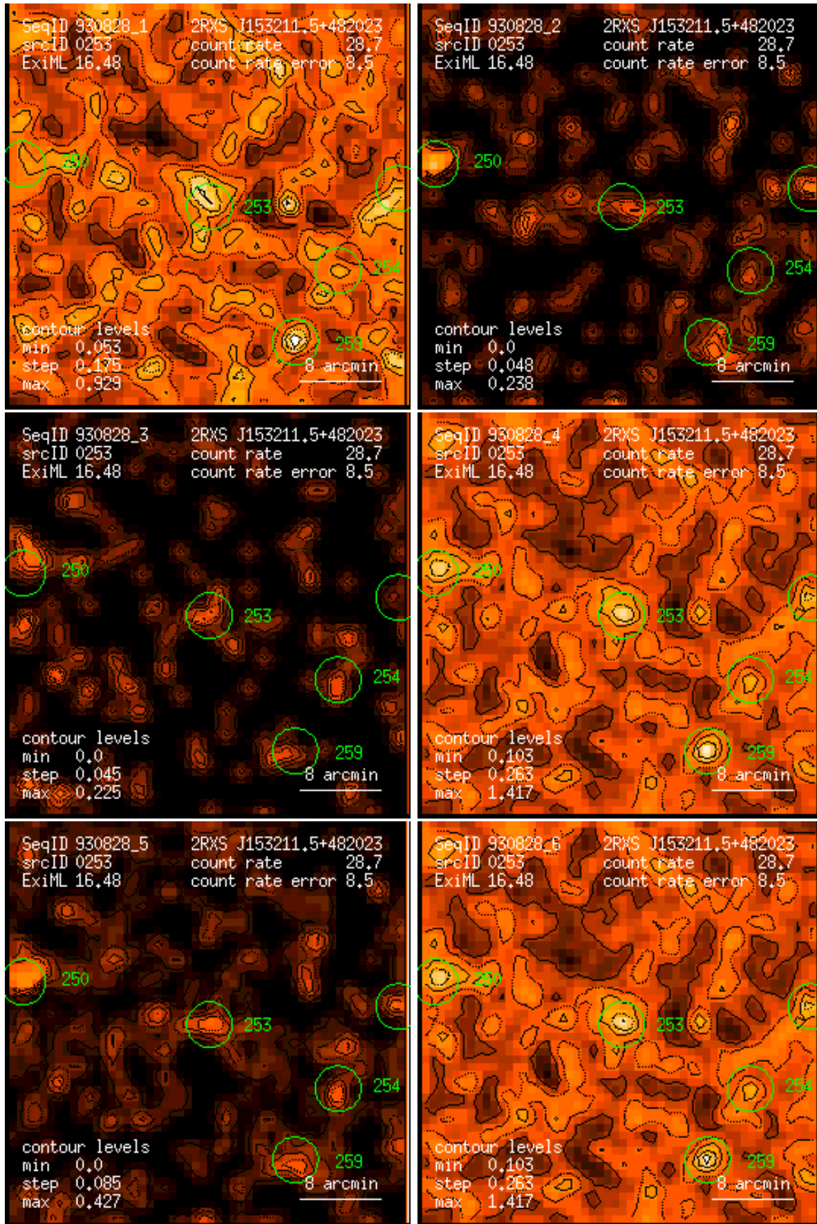
Figure 253: RASS 930828: detection 0253: band rate images, Gaussian filter: (1) PSPC channels 11 – 41, (2) 52 – 90, (3) 91 – 201, (4) 11 – 235, (5) 52 – 201, (6) 11 – 201. Broad band rates in counts/ks. Band rate contour levels in counts/ks/arcmin 2 .
