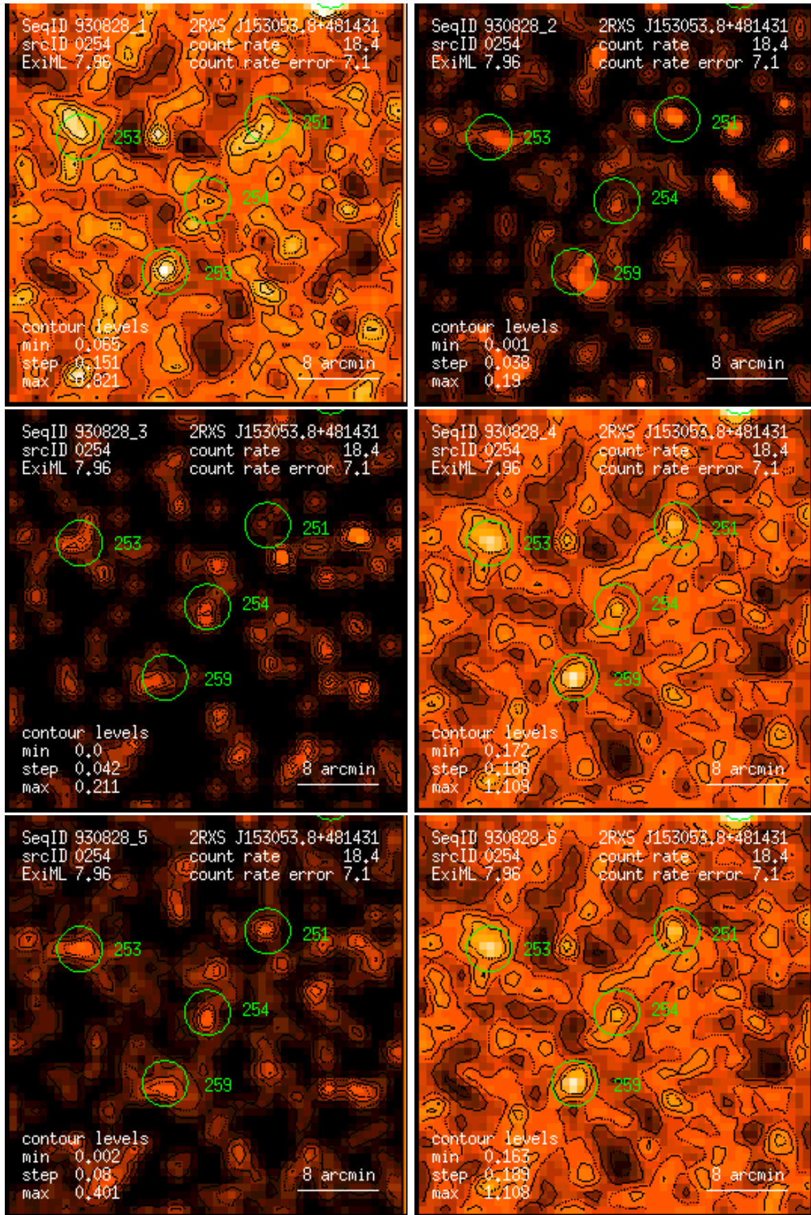
Figure 254: RASS 930828: detection 0254: band rate images, Gaussian filter: (1) PSPC channels 11 – 41, (2) 52 – 90, (3) 91 – 201, (4) 11 – 235, (5) 52 – 201, (6) 11 – 201. Broad band rates in counts/ks. Band rate contour levels in counts/ks/arcmin 2 .
