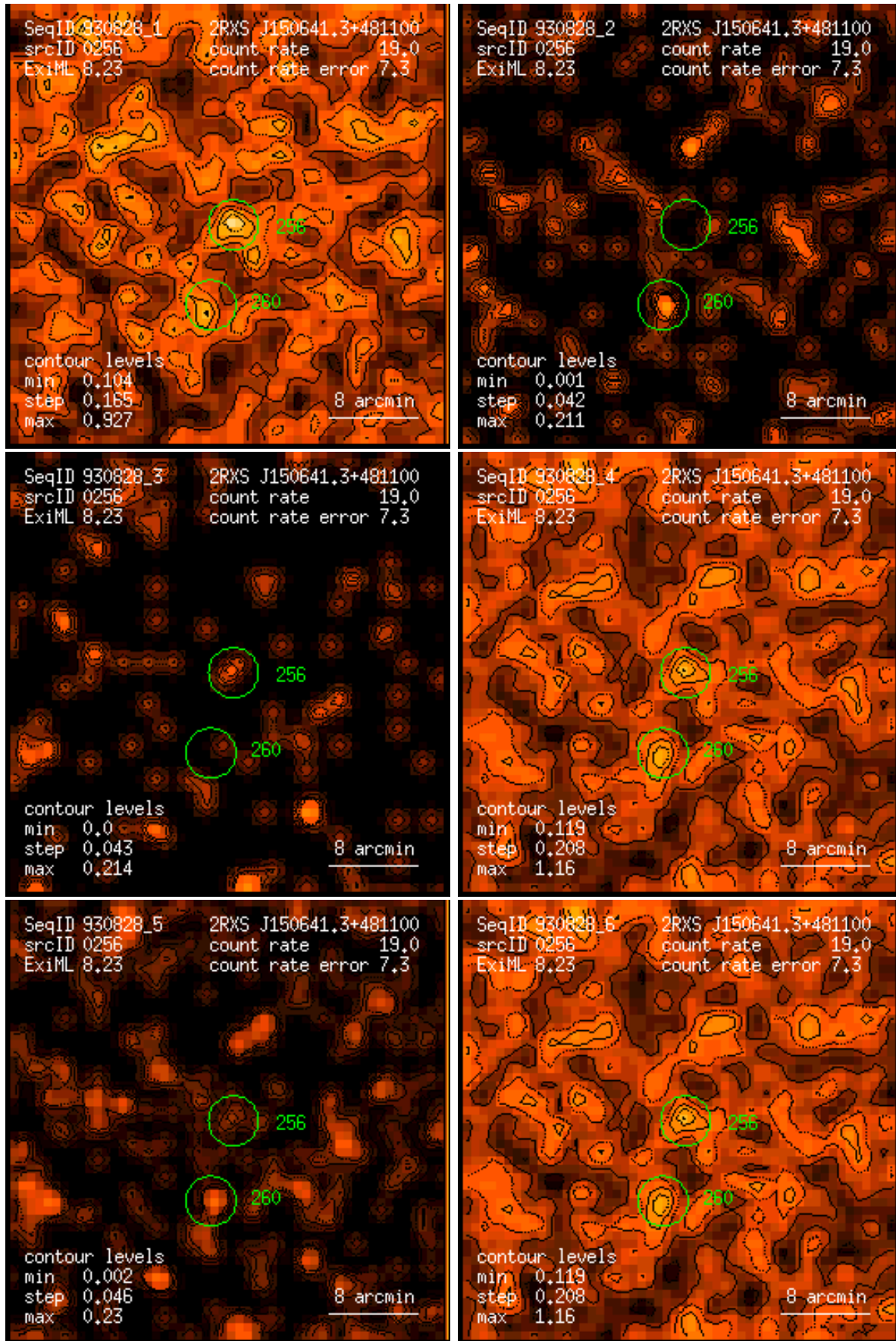
Figure 256: RASS 930828: detection 0256: band rate images, Gaussian filter: (1) PSPC channels 11 – 41, (2) 52 – 90, (3) 91 – 201, (4) 11 – 235, (5) 52 – 201, (6) 11 – 201. Broad band rates in counts/ks. Band rate contour levels in counts/ks/arcmin 2 .
