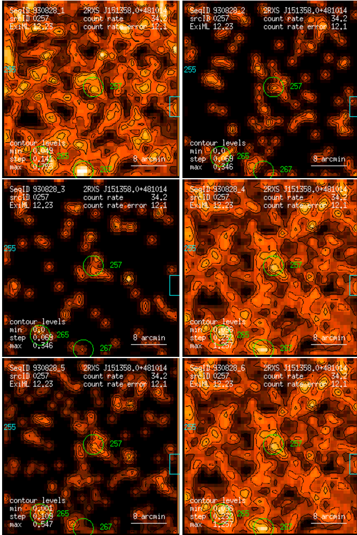
Figure 257: RASS 930828: detection 0257: band rate images, Gaussian filter: (1) PSPC channels 11 – 41, (2) 52 – 90, (3) 91 – 201, (4) 11 – 235, (5) 52 – 201, (6) 11 – 201. Broad band rates in counts/ks. Band rate contour levels in counts/ks/arcmin 2 .
