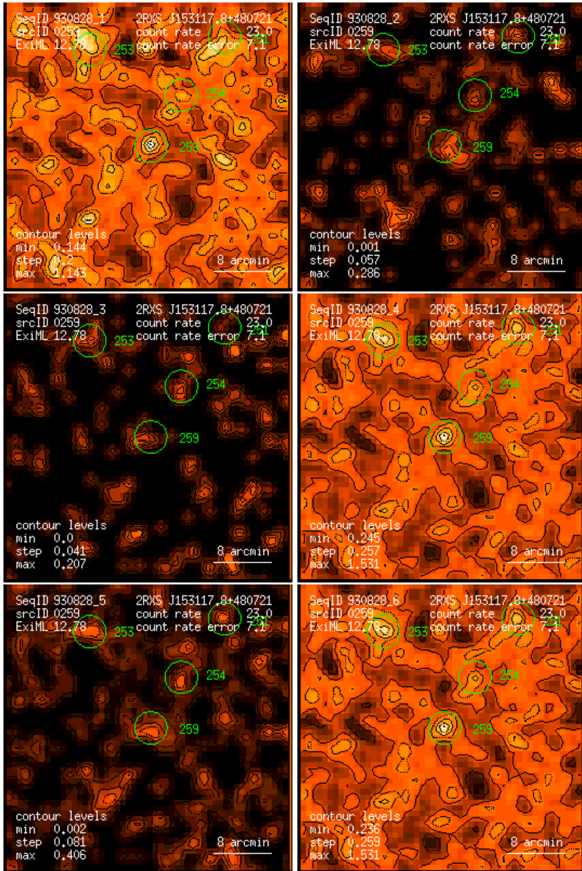
Figure 259: RASS 930828: detection 0259: band rate images, Gaussian filter: (1) PSPC channels 11 – 41, (2) 52 – 90, (3) 91 – 201, (4) 11 – 235, (5) 52 – 201, (6) 11 – 201. Broad band rates in counts/ks. Band rate contour levels in counts/ks/arcmin 2 .
