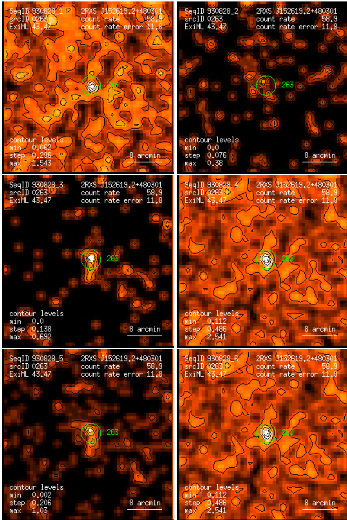
Figure 263: RASS 930828: detection 0263: band rate images, Gaussian filter: (1) PSPC channels 11 – 41, (2) 52 – 90, (3) 91 – 201, (4) 11 – 235, (5) 52 – 201, (6) 11 – 201. Broad band rates in counts/ks. Band rate contour levels in counts/ks/arcmin 2 .
