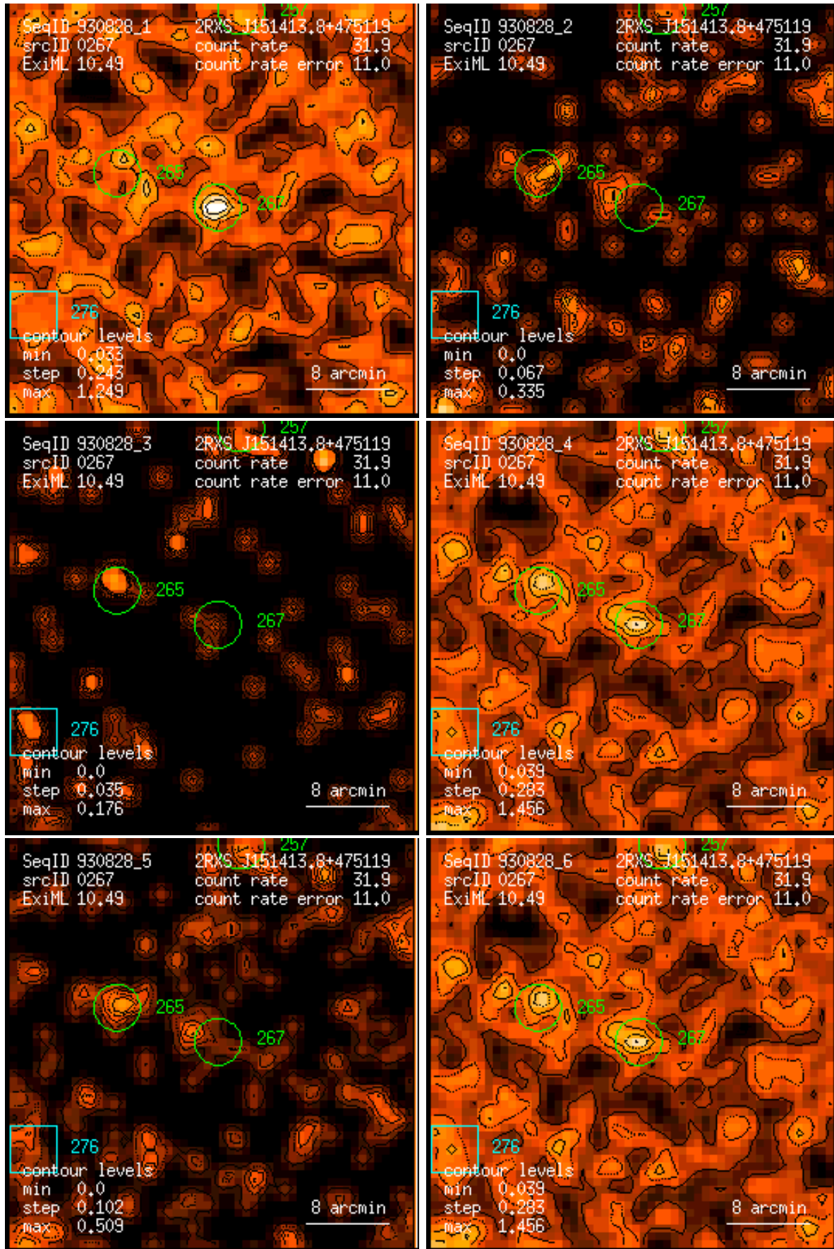
Figure 267: RASS 930828: detection 0267: band rate images, Gaussian filter: (1) PSPC channels 11 – 41, (2) 52 – 90, (3) 91 – 201, (4) 11 – 235, (5) 52 – 201, (6) 11 – 201. Broad band rates in counts/ks. Band rate contour levels in counts/ks/arcmin 2 .
