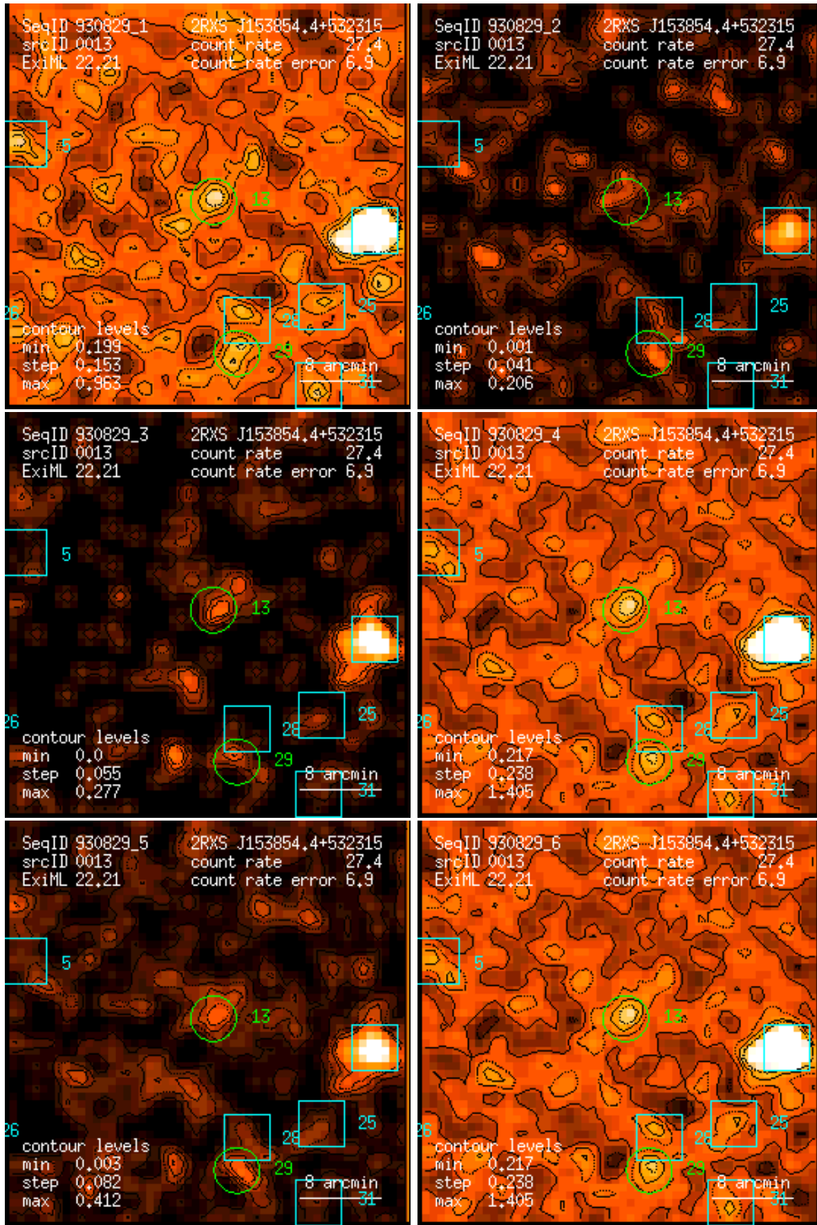
Figure 13: RASS 930829: detection 0013: band rate images, Gaussian filter: (1) PSPC channels 11 – 41, (2) 52 – 90, (3) 91 – 201, (4) 11 – 235, (5) 52 – 201, (6) 11 – 201. Broad band rates in counts/ks. Band rate contour levels in counts/ks/arcmin 2 .
