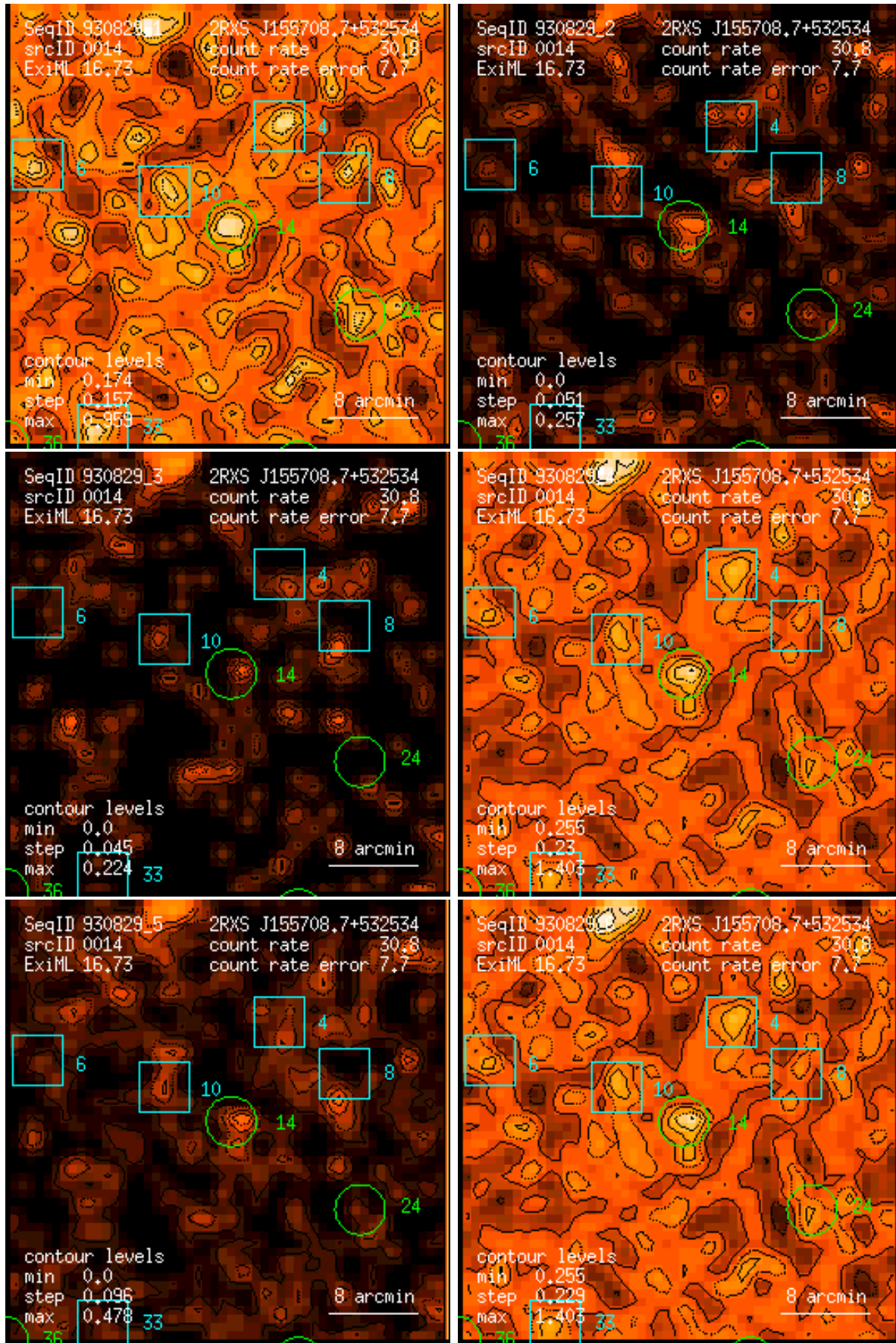
Figure 14: RASS 930829: detection 0014: band rate images, Gaussian filter: (1) PSPC channels 11 – 41, (2) 52 – 90, (3) 91 – 201, (4) 11 – 235, (5) 52 – 201, (6) 11 – 201. Broad band rates in counts/ks. Band rate contour levels in counts/ks/arcmin 2 .
