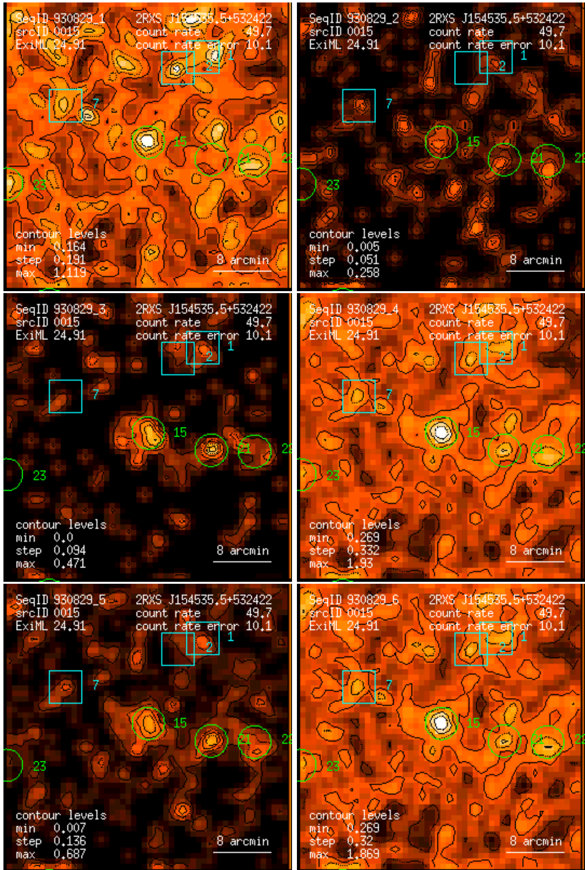
Figure 15: RASS 930829: detection 0015: band rate images, Gaussian filter: (1) PSPC channels 11 – 41, (2) 52 – 90, (3) 91 – 201, (4) 11 – 235, (5) 52 – 201, (6) 11 – 201. Broad band rates in counts/ks. Band rate contour levels in counts/ks/arcmin 2 .
