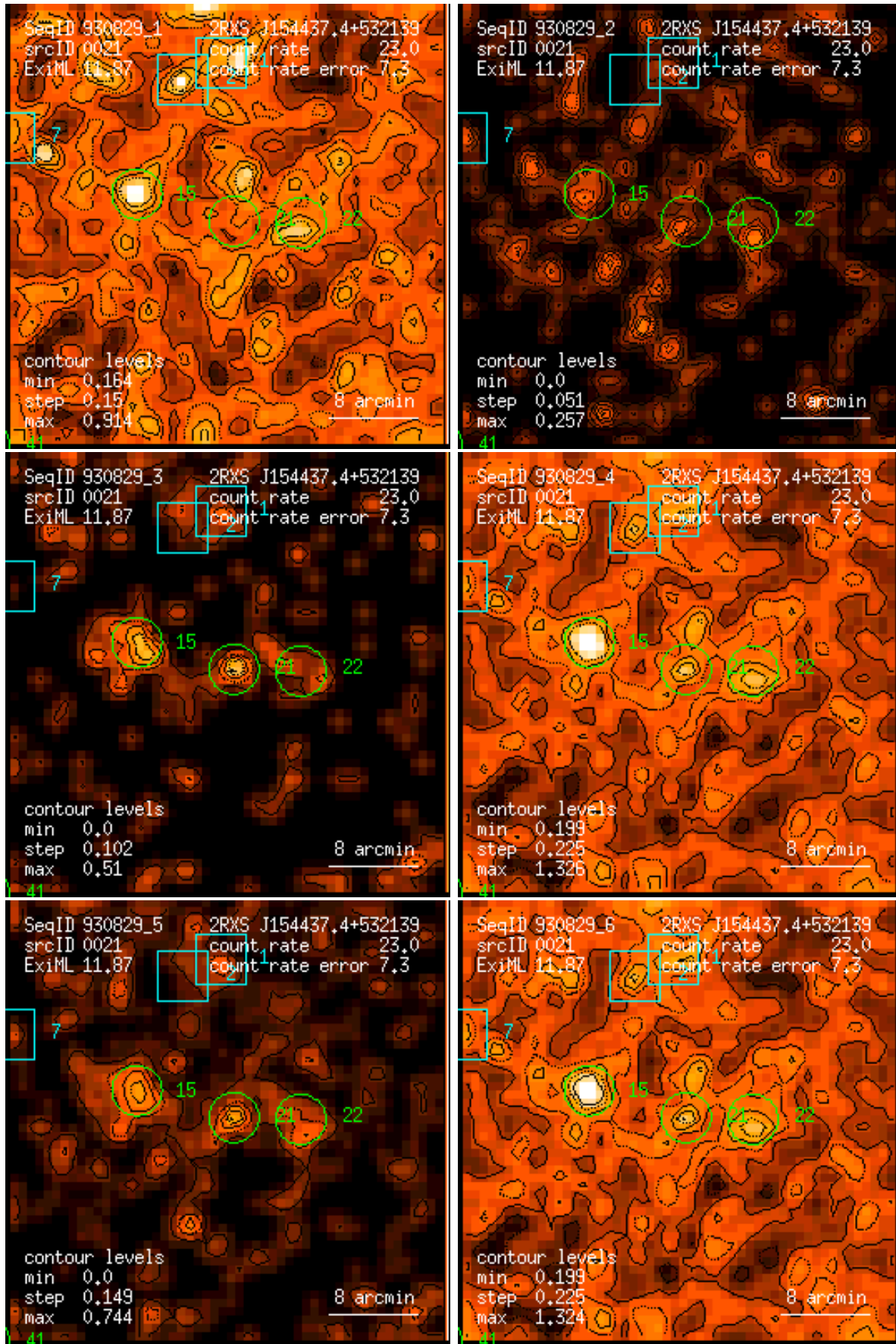
Figure 21: RASS 930829: detection 0021: band rate images, Gaussian filter: (1) PSPC channels 11 – 41, (2) 52 – 90, (3) 91 – 201, (4) 11 – 235, (5) 52 – 201, (6) 11 – 201. Broad band rates in counts/ks. Band rate contour levels in counts/ks/arcmin 2 .
