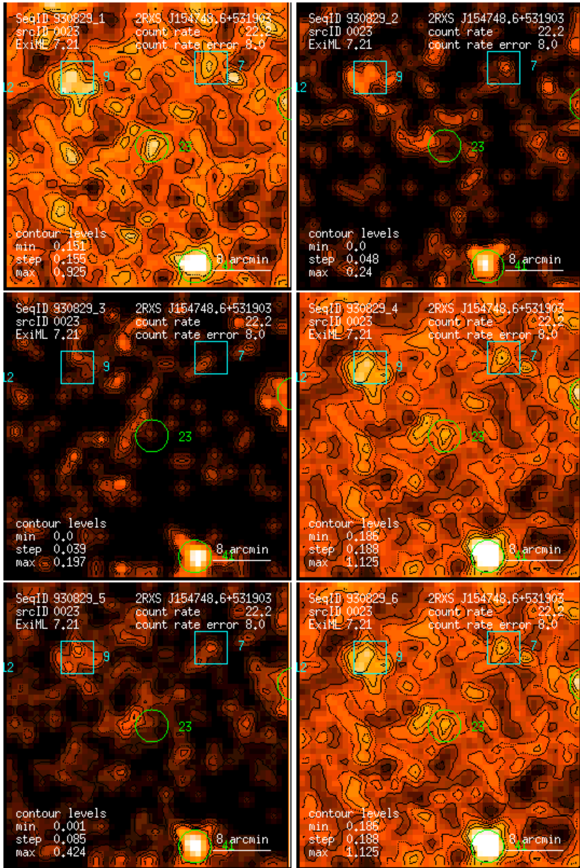
Figure 23: RASS 930829: detection 0023: band rate images, Gaussian filter: (1) PSPC channels 11 – 41, (2) 52 – 90, (3) 91 – 201, (4) 11 – 235, (5) 52 – 201, (6) 11 – 201. Broad band rates in counts/ks. Band rate contour levels in counts/ks/arcmin 2 .
