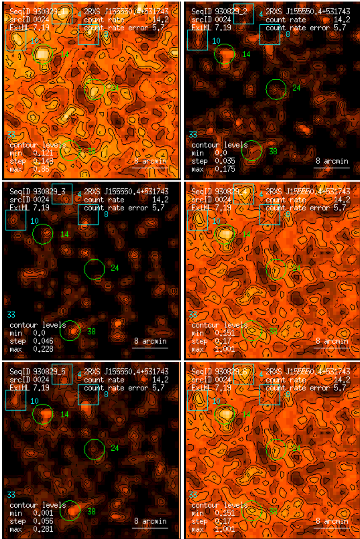
Figure 24: RASS 930829: detection 0024: band rate images, Gaussian filter: (1) PSPC channels 11 – 41, (2) 52 – 90, (3) 91 – 201, (4) 11 – 235, (5) 52 – 201, (6) 11 – 201. Broad band rates in counts/ks. Band rate contour levels in counts/ks/arcmin 2 .
