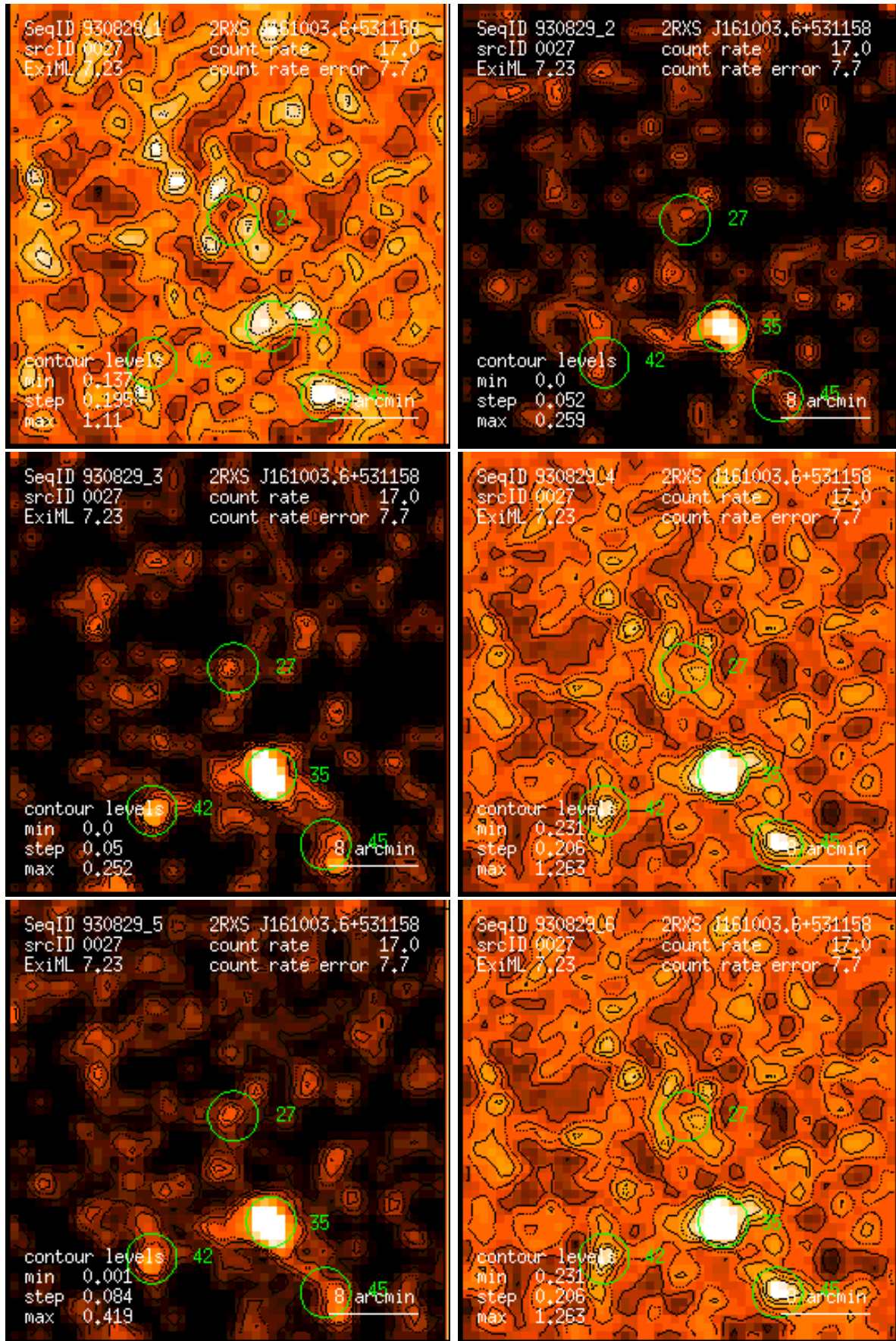
Figure 27: RASS 930829: detection 0027: band rate images, Gaussian filter: (1) PSPC channels 11 – 41, (2) 52 – 90, (3) 91 – 201, (4) 11 – 235, (5) 52 – 201, (6) 11 – 201. Broad band rates in counts/ks. Band rate contour levels in counts/ks/arcmin 2 .
