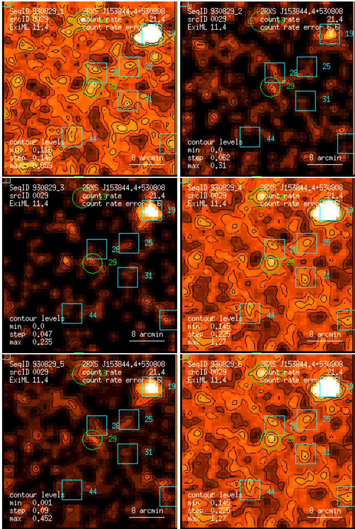
Figure 29: RASS 930829: detection 0029: band rate images, Gaussian filter: (1) PSPC channels 11 – 41, (2) 52 – 90, (3) 91 – 201, (4) 11 – 235, (5) 52 – 201, (6) 11 – 201. Broad band rates in counts/ks. Band rate contour levels in counts/ks/arcmin 2 .
