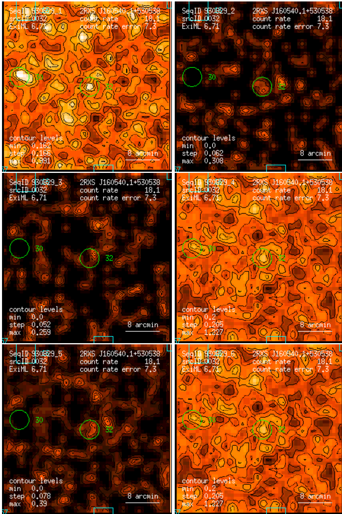
Figure 32: RASS 930829: detection 0032: band rate images, Gaussian filter: (1) PSPC channels 11 – 41, (2) 52 – 90, (3) 91 – 201, (4) 11 – 235, (5) 52 – 201, (6) 11 – 201. Broad band rates in counts/ks. Band rate contour levels in counts/ks/arcmin 2 .
