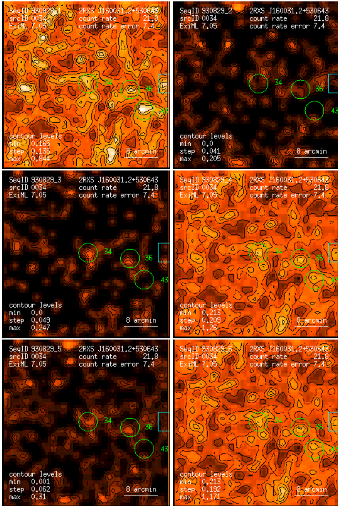
Figure 34: RASS 930829: detection 0034: band rate images, Gaussian filter: (1) PSPC channels 11 – 41, (2) 52 – 90, (3) 91 – 201, (4) 11 – 235, (5) 52 – 201, (6) 11 – 201. Broad band rates in counts/ks. Band rate contour levels in counts/ks/arcmin 2 .
