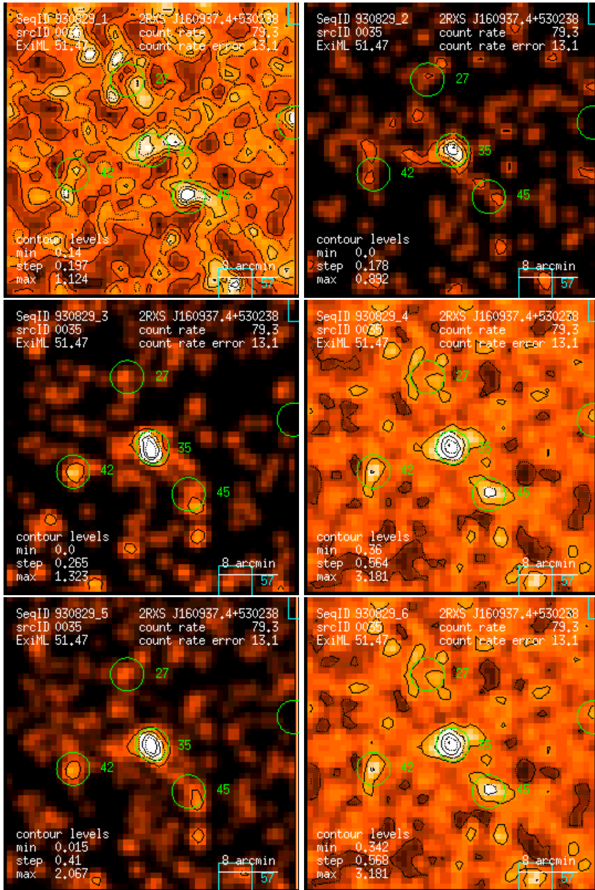
Figure 35: RASS 930829: detection 0035: band rate images, Gaussian filter: (1) PSPC channels 11 – 41, (2) 52 – 90, (3) 91 – 201, (4) 11 – 235, (5) 52 – 201, (6) 11 – 201. Broad band rates in counts/ks. Band rate contour levels in counts/ks/arcmin 2 .
