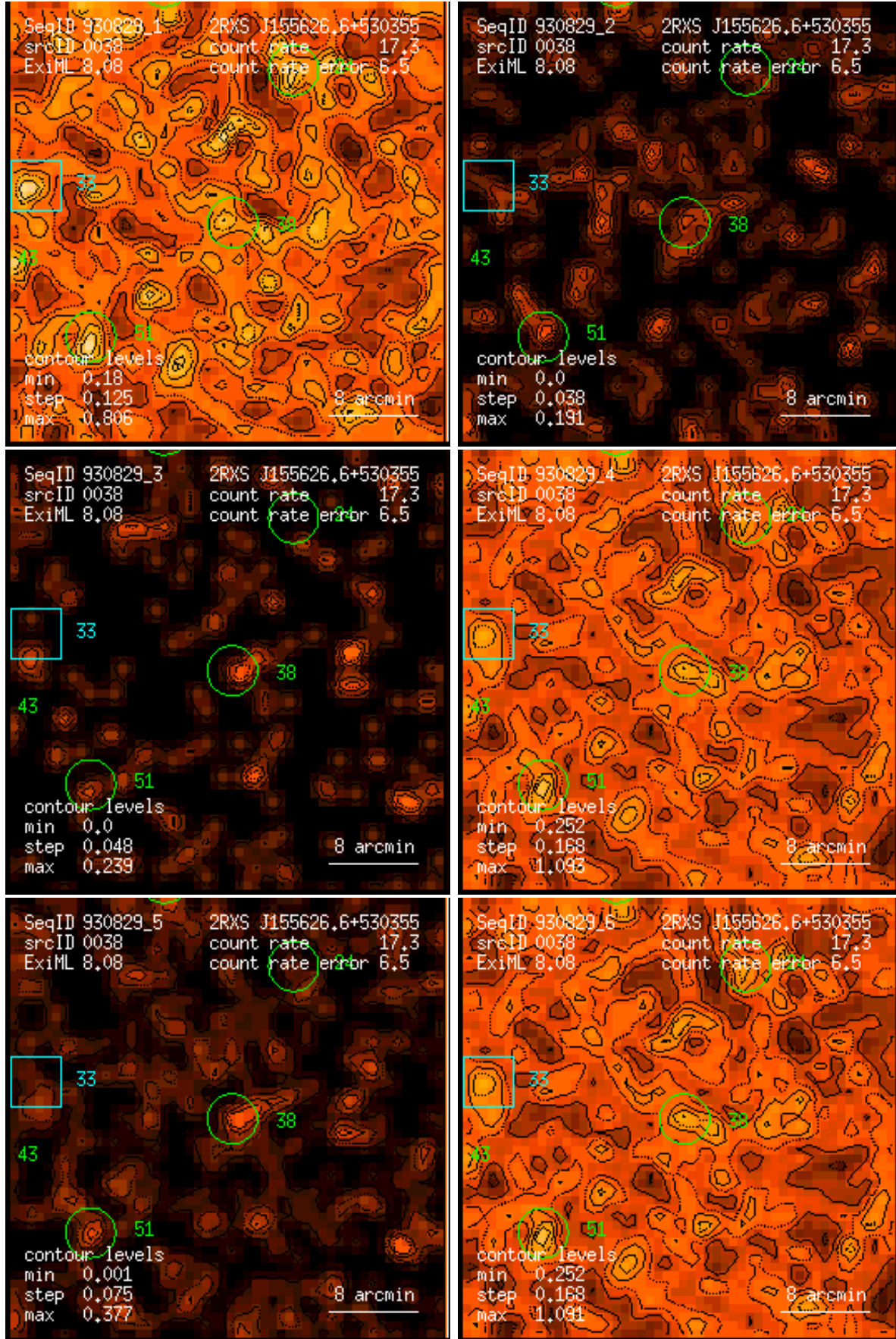
Figure 38: RASS 930829: detection 0038: band rate images, Gaussian filter: (1) PSPC channels 11 – 41, (2) 52 – 90, (3) 91 – 201, (4) 11 – 235, (5) 52 – 201, (6) 11 – 201. Broad band rates in counts/ks. Band rate contour levels in counts/ks/arcmin 2 .
