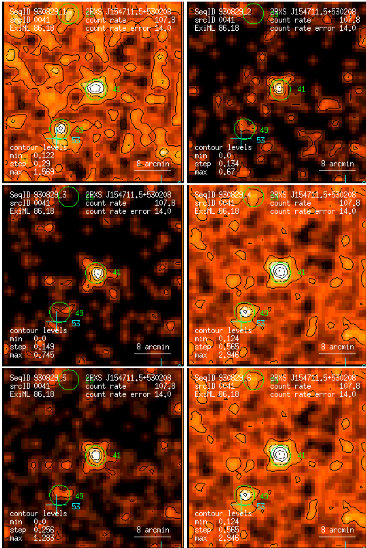
Figure 41: RASS 930829: detection 0041: band rate images, Gaussian filter: (1) PSPC channels 11 – 41, (2) 52 – 90, (3) 91 – 201, (4) 11 – 235, (5) 52 – 201, (6) 11 – 201. Broad band rates in counts/ks. Band rate contour levels in counts/ks/arcmin 2 .
