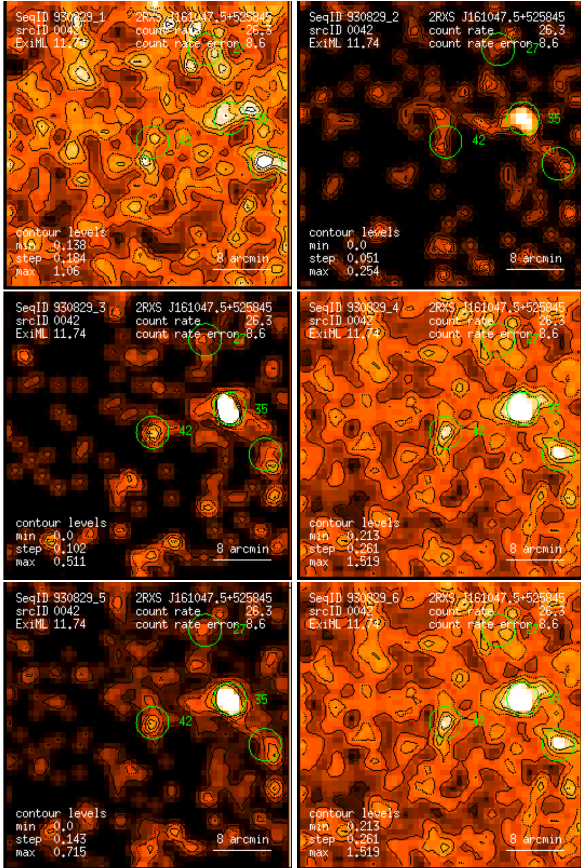
Figure 42: RASS 930829: detection 0042: band rate images, Gaussian filter: (1) PSPC channels 11 – 41, (2) 52 – 90, (3) 91 – 201, (4) 11 – 235, (5) 52 – 201, (6) 11 – 201. Broad band rates in counts/ks. Band rate contour levels in counts/ks/arcmin 2 .
