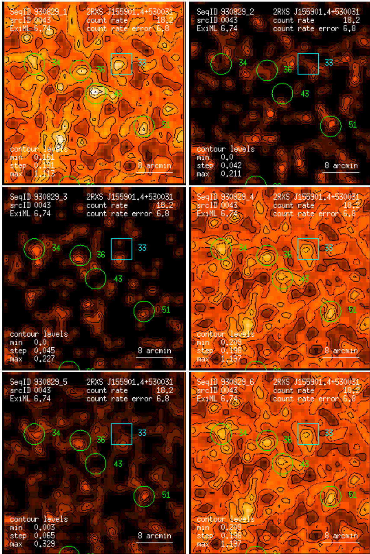
Figure 43: RASS 930829: detection 0043: band rate images, Gaussian filter: (1) PSPC channels 11 – 41, (2) 52 – 90, (3) 91 – 201, (4) 11 – 235, (5) 52 – 201, (6) 11 – 201. Broad band rates in counts/ks. Band rate contour levels in counts/ks/arcmin 2 .
