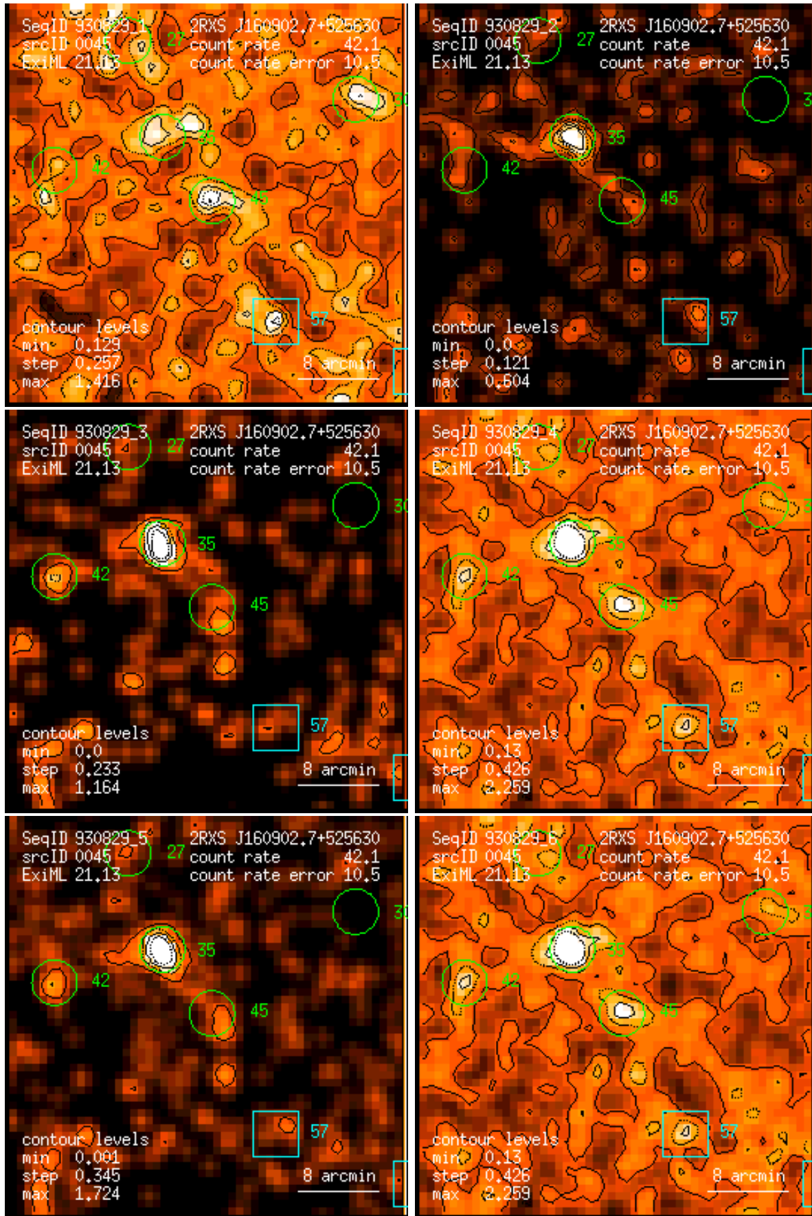
Figure 45: RASS 930829: detection 0045: band rate images, Gaussian filter: (1) PSPC channels 11 – 41, (2) 52 – 90, (3) 91 – 201, (4) 11 – 235, (5) 52 – 201, (6) 11 – 201. Broad band rates in counts/ks. Band rate contour levels in counts/ks/arcmin 2 .
