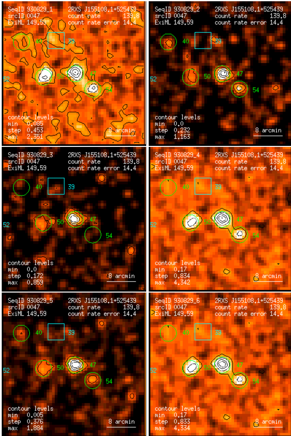
Figure 47: RASS 930829: detection 0047: band rate images, Gaussian filter: (1) PSPC channels 11 – 41, (2) 52 – 90, (3) 91 – 201, (4) 11 – 235, (5) 52 – 201, (6) 11 – 201. Broad band rates in counts/ks. Band rate contour levels in counts/ks/arcmin 2 .
