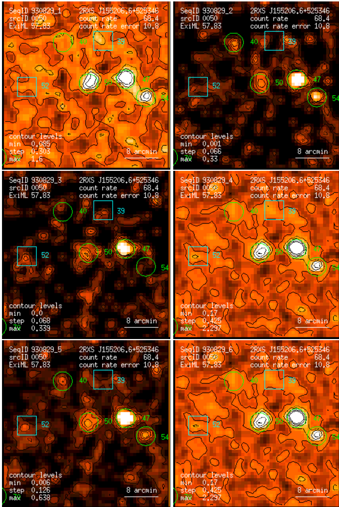
Figure 50: RASS 930829: detection 0050: band rate images, Gaussian filter: (1) PSPC channels 11 – 41, (2) 52 – 90, (3) 91 – 201, (4) 11 – 235, (5) 52 – 201, (6) 11 – 201. Broad band rates in counts/ks. Band rate contour levels in counts/ks/arcmin 2 .
