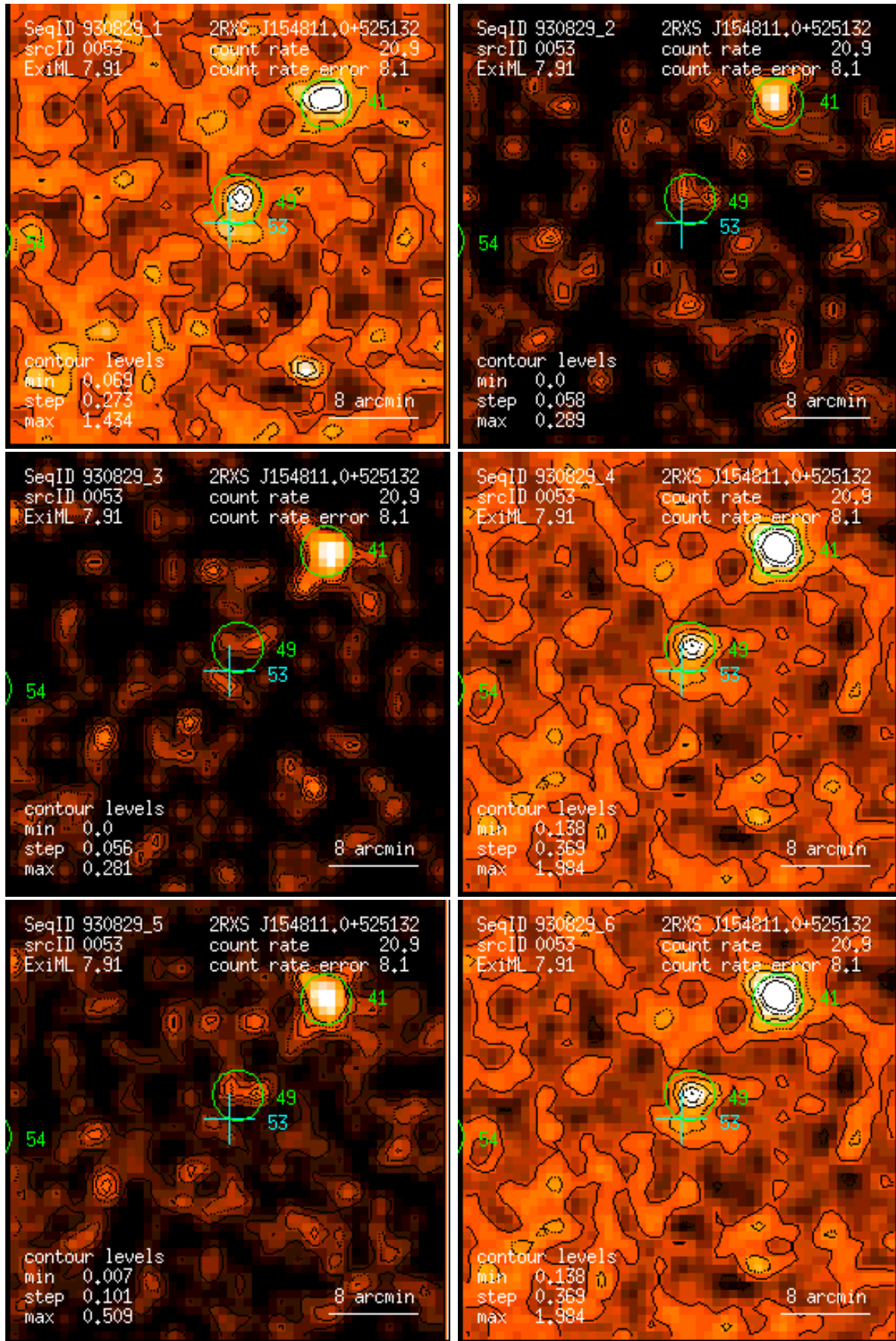
Figure 53: RASS 930829: detection 0053: band rate images, Gaussian filter: (1) PSPC channels 11 – 41, (2) 52 – 90, (3) 91 – 201, (4) 11 – 235, (5) 52 – 201, (6) 11 – 201. Broad band rates in counts/ks. Band rate contour levels in counts/ks/arcmin 2 .
