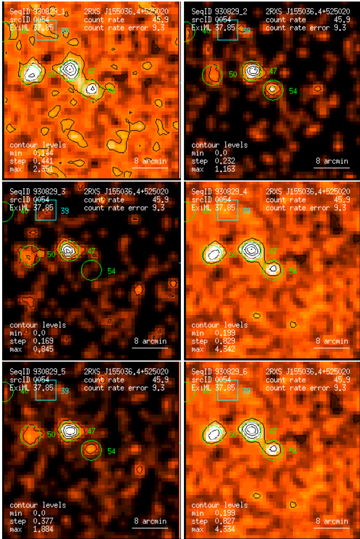
Figure 54: RASS 930829: detection 0054: band rate images, Gaussian filter: (1) PSPC channels 11 – 41, (2) 52 – 90, (3) 91 – 201, (4) 11 – 235, (5) 52 – 201, (6) 11 – 201. Broad band rates in counts/ks. Band rate contour levels in counts/ks/arcmin 2 .
