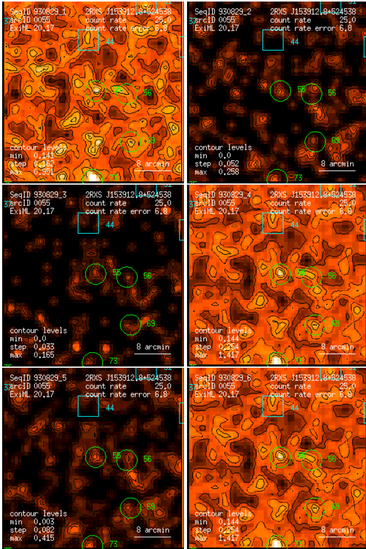
Figure 55: RASS 930829: detection 0055: band rate images, Gaussian filter: (1) PSPC channels 11 – 41, (2) 52 – 90, (3) 91 – 201, (4) 11 – 235, (5) 52 – 201, (6) 11 – 201. Broad band rates in counts/ks. Band rate contour levels in counts/ks/arcmin 2 .
