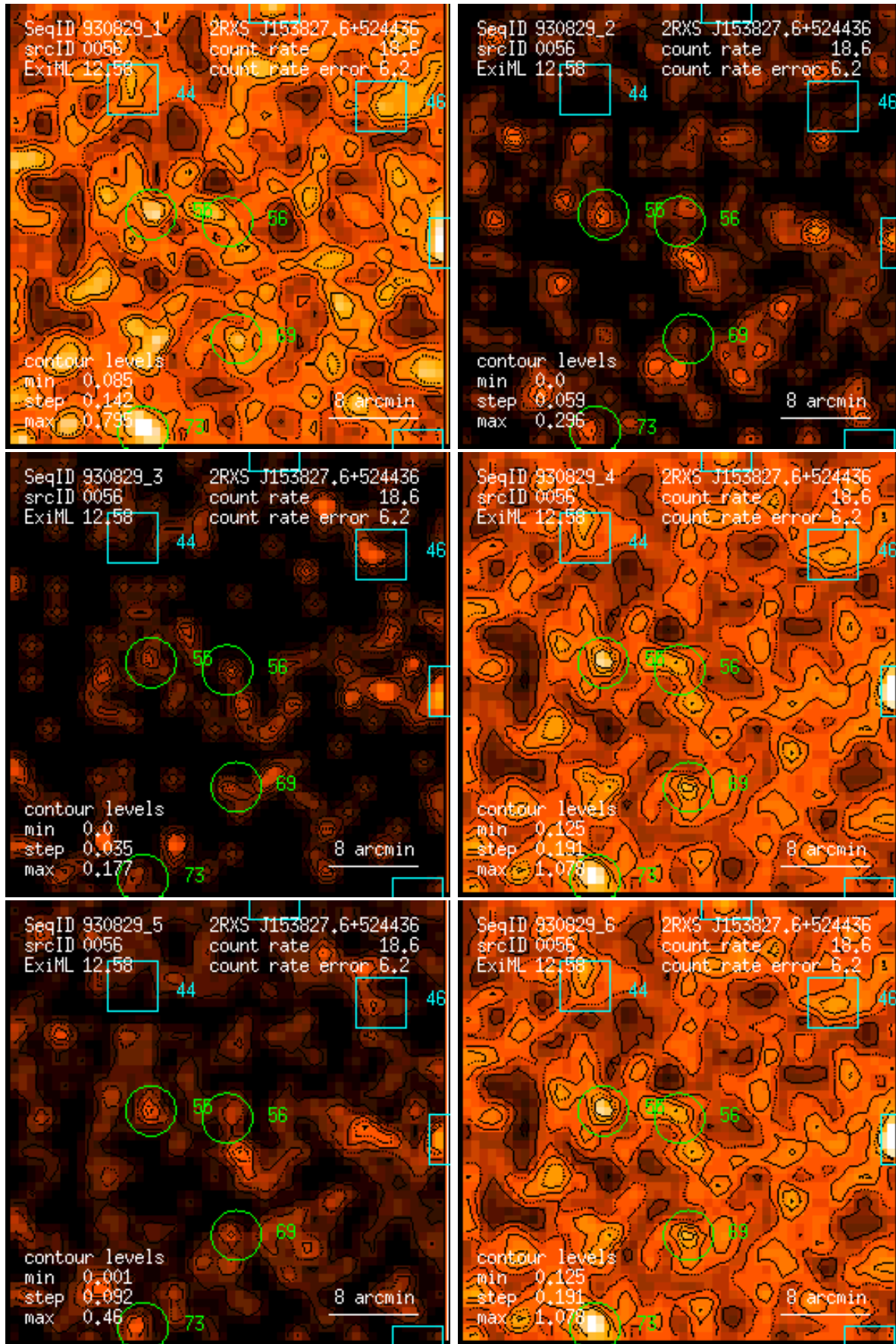
Figure 56: RASS 930829: detection 0056: band rate images, Gaussian filter: (1) PSPC channels 11 – 41, (2) 52 – 90, (3) 91 – 201, (4) 11 – 235, (5) 52 – 201, (6) 11 – 201. Broad band rates in counts/ks. Band rate contour levels in counts/ks/arcmin 2 .
