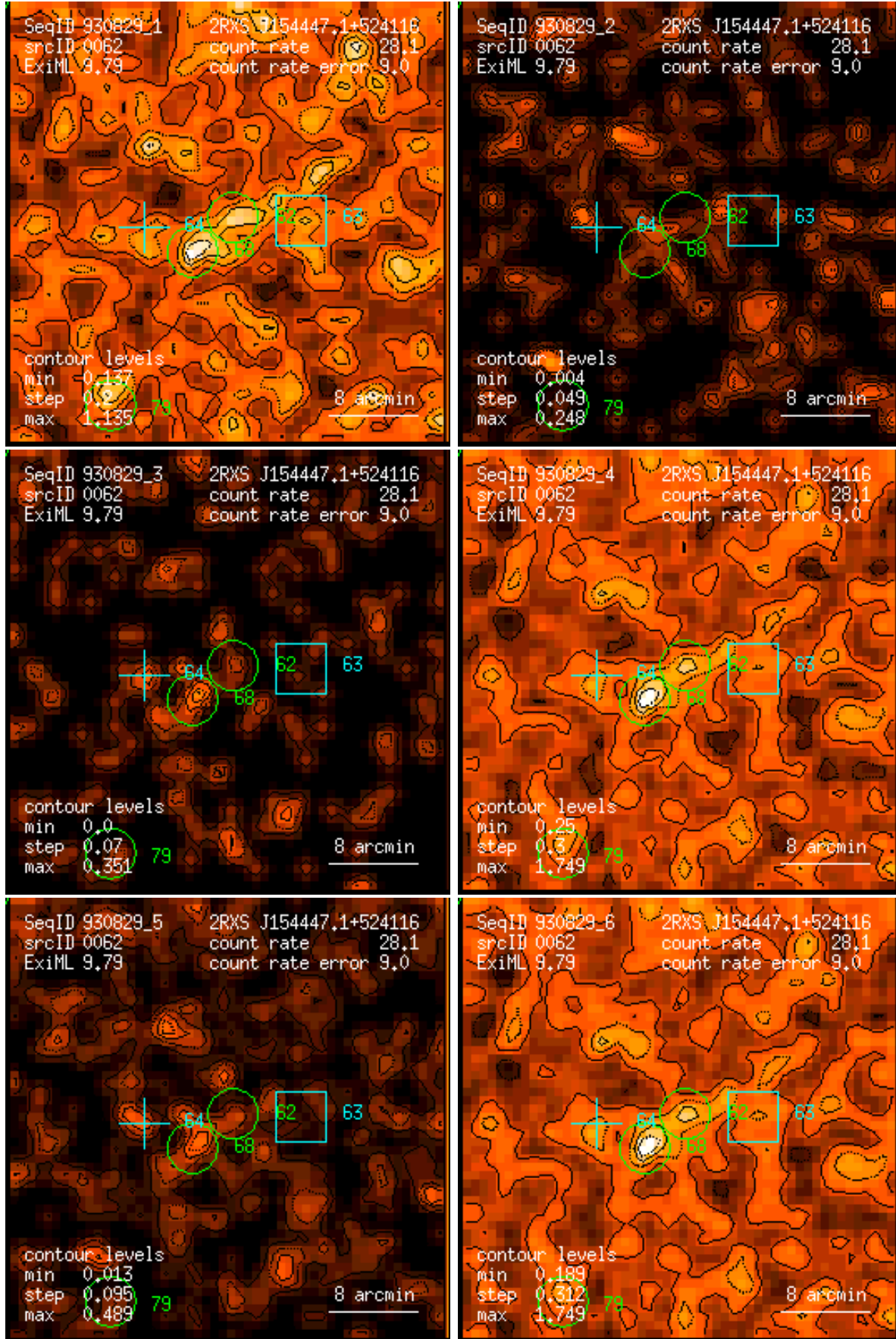
Figure 62: RASS 930829: detection 0062: band rate images, Gaussian filter: (1) PSPC channels 11 – 41, (2) 52 – 90, (3) 91 – 201, (4) 11 – 235, (5) 52 – 201, (6) 11 – 201. Broad band rates in counts/ks. Band rate contour levels in counts/ks/arcmin 2 .
