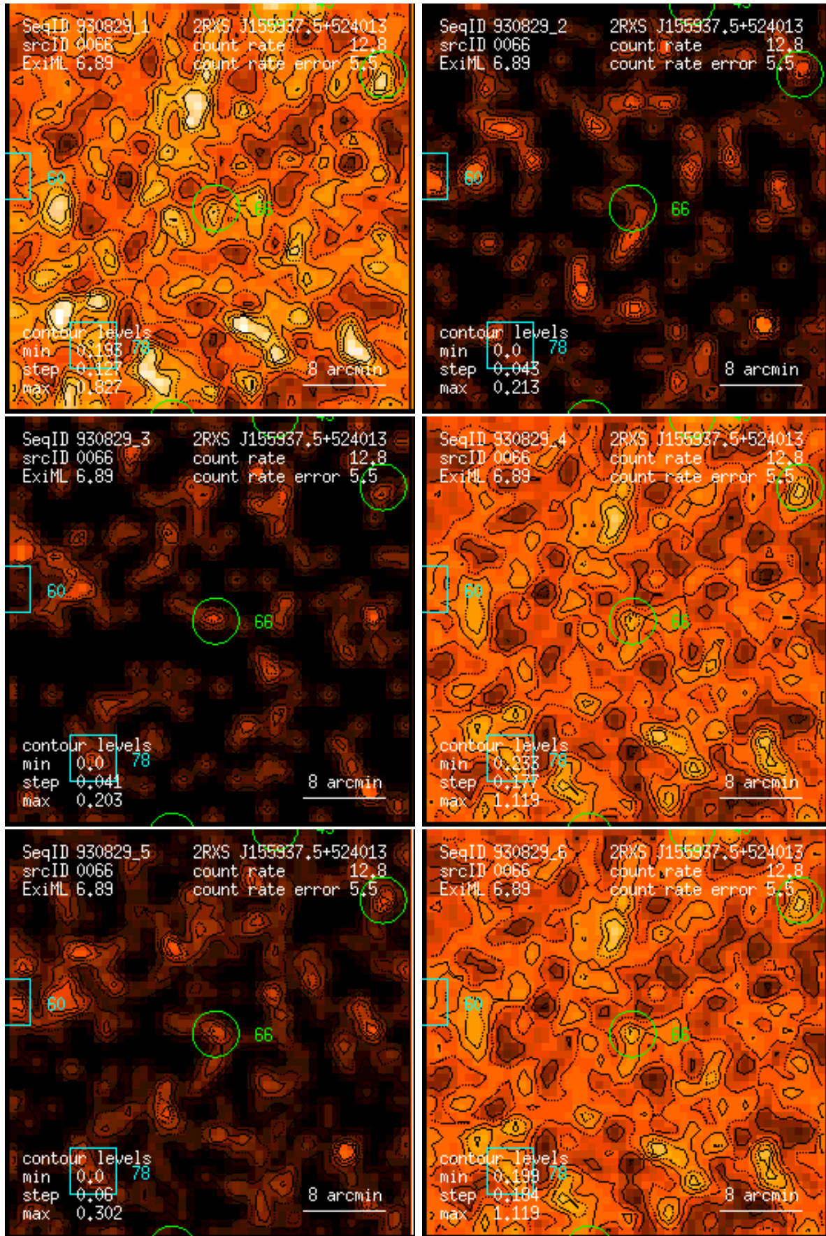
Figure 66: RASS 930829: detection 0066: band rate images, Gaussian filter: (1) PSPC channels 11 – 41, (2) 52 – 90, (3) 91 – 201, (4) 11 – 235, (5) 52 – 201, (6) 11 – 201. Broad band rates in counts/ks. Band rate contour levels in counts/ks/arcmin 2 .
