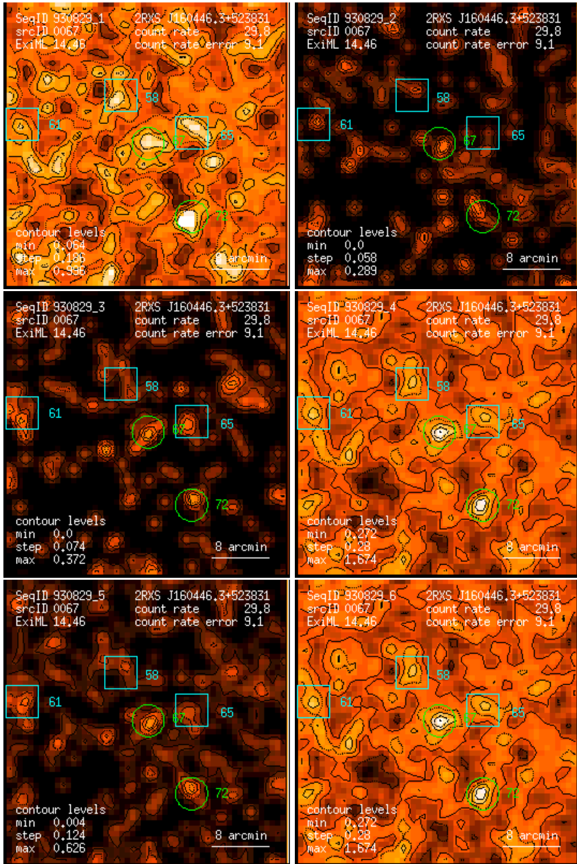
Figure 67: RASS 930829: detection 0067: band rate images, Gaussian filter: (1) PSPC channels 11 – 41, (2) 52 – 90, (3) 91 – 201, (4) 11 – 235, (5) 52 – 201, (6) 11 – 201. Broad band rates in counts/ks. Band rate contour levels in counts/ks/arcmin 2 .
