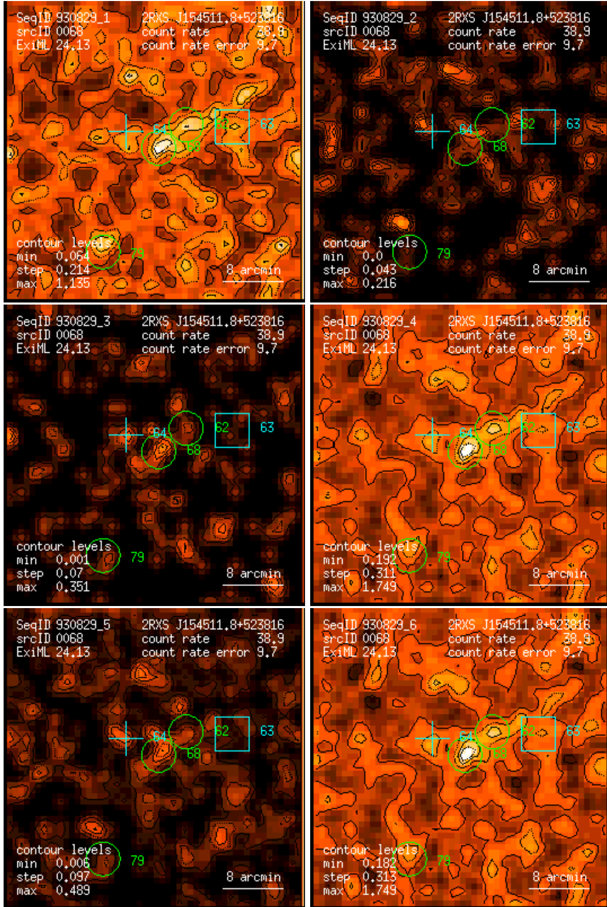
Figure 68: RASS 930829: detection 0068: band rate images, Gaussian filter: (1) PSPC channels 11 – 41, (2) 52 – 90, (3) 91 – 201, (4) 11 – 235, (5) 52 – 201, (6) 11 – 201. Broad band rates in counts/ks. Band rate contour levels in counts/ks/arcmin 2 .
