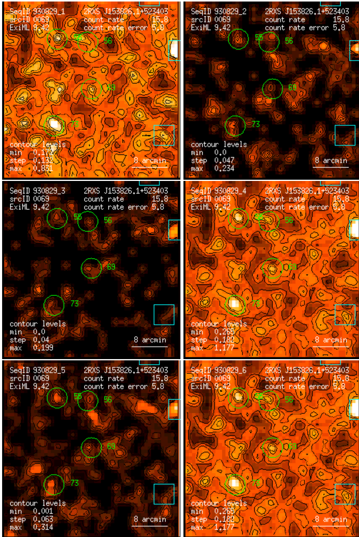
Figure 69: RASS 930829: detection 0069: band rate images, Gaussian filter: (1) PSPC channels 11 – 41, (2) 52 – 90, (3) 91 – 201, (4) 11 – 235, (5) 52 – 201, (6) 11 – 201. Broad band rates in counts/ks. Band rate contour levels in counts/ks/arcmin 2 .
