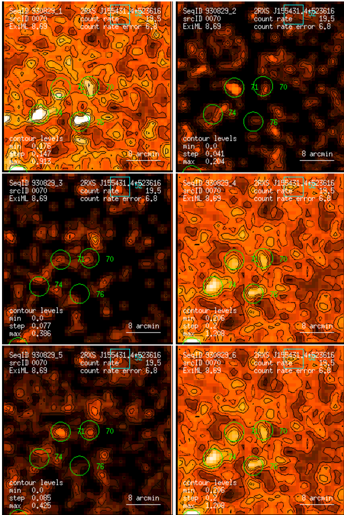
Figure 70: RASS 930829: detection 0070: band rate images, Gaussian filter: (1) PSPC channels 11 – 41, (2) 52 – 90, (3) 91 – 201, (4) 11 – 235, (5) 52 – 201, (6) 11 – 201. Broad band rates in counts/ks. Band rate contour levels in counts/ks/arcmin 2 .
