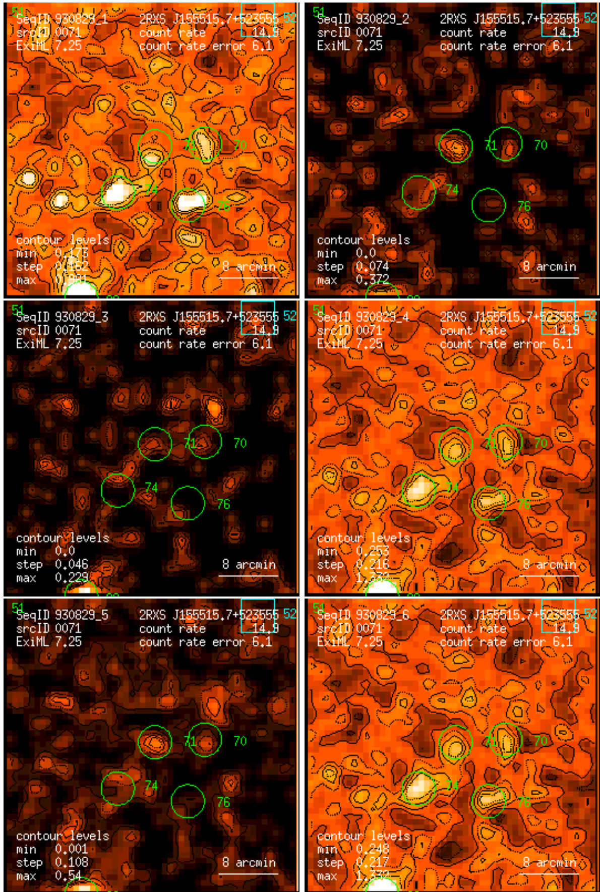
Figure 71: RASS 930829: detection 0071: band rate images, Gaussian filter: (1) PSPC channels 11 – 41, (2) 52 – 90, (3) 91 – 201, (4) 11 – 235, (5) 52 – 201, (6) 11 – 201. Broad band rates in counts/ks. Band rate contour levels in counts/ks/arcmin 2 .
