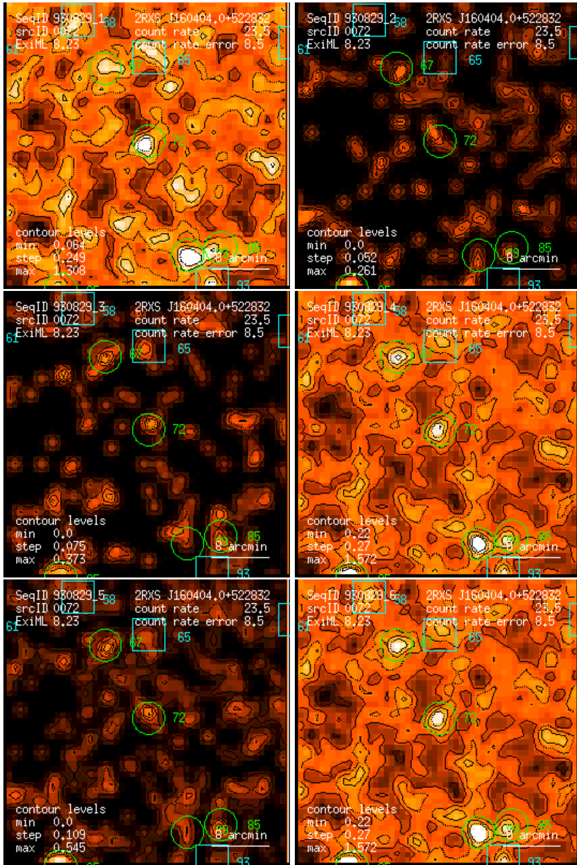
Figure 72: RASS 930829: detection 0072: band rate images, Gaussian filter: (1) PSPC channels 11 – 41, (2) 52 – 90, (3) 91 – 201, (4) 11 – 235, (5) 52 – 201, (6) 11 – 201. Broad band rates in counts/ks. Band rate contour levels in counts/ks/arcmin 2 .
