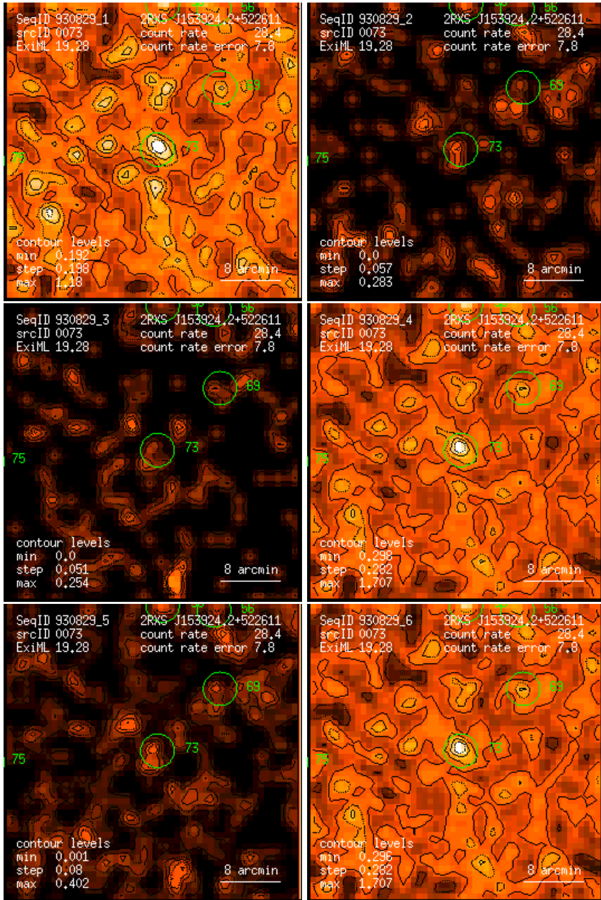
Figure 73: RASS 930829: detection 0073: band rate images, Gaussian filter: (1) PSPC channels 11 – 41, (2) 52 – 90, (3) 91 – 201, (4) 11 – 235, (5) 52 – 201, (6) 11 – 201. Broad band rates in counts/ks. Band rate contour levels in counts/ks/arcmin 2 .
