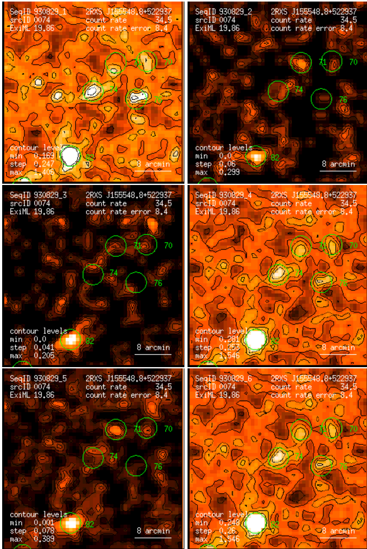
Figure 74: RASS 930829: detection 0074: band rate images, Gaussian filter: (1) PSPC channels 11 – 41, (2) 52 – 90, (3) 91 – 201, (4) 11 – 235, (5) 52 – 201, (6) 11 – 201. Broad band rates in counts/ks. Band rate contour levels in counts/ks/arcmin 2 .
